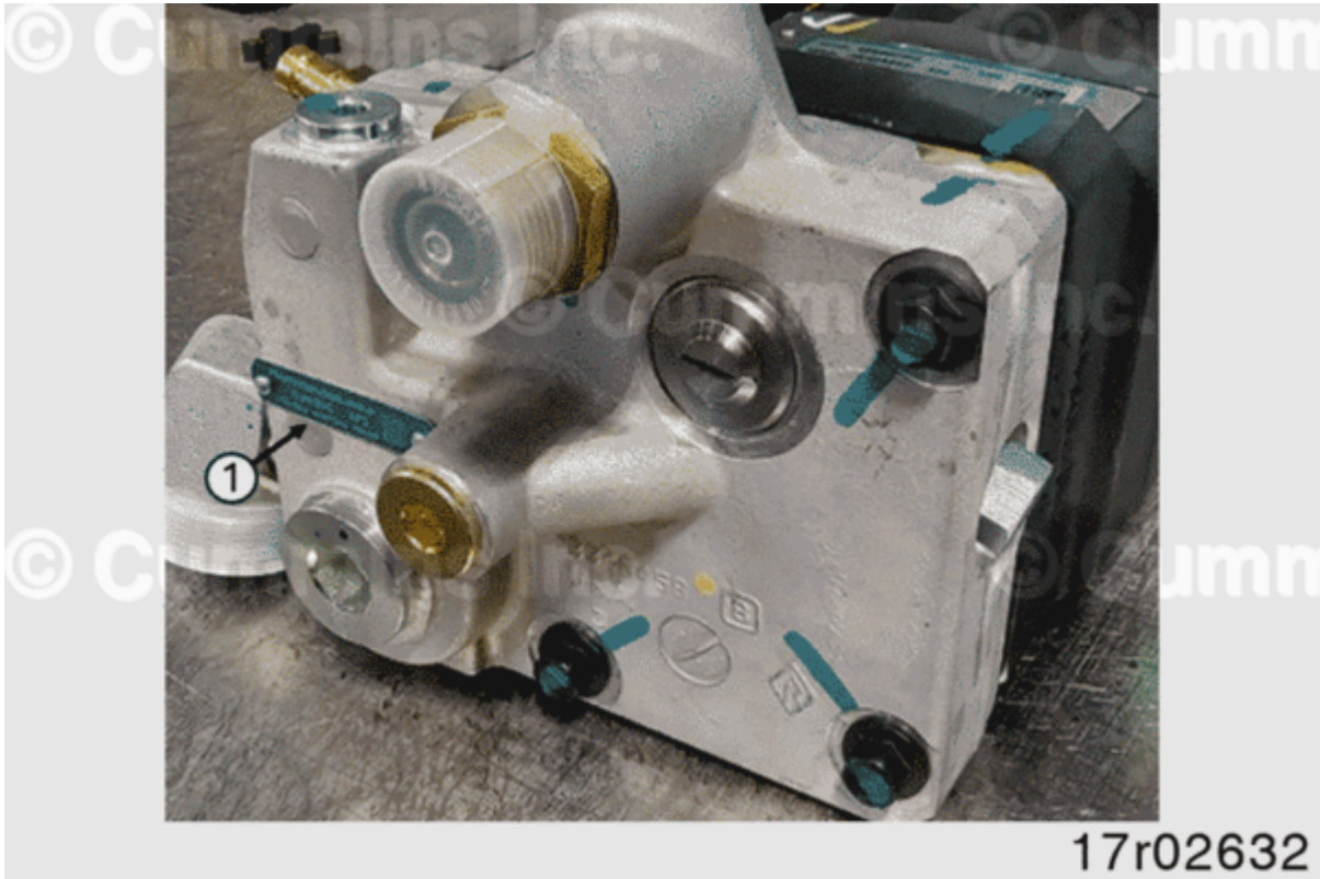
Figure 1, Assembly with fuel pump serial number location
