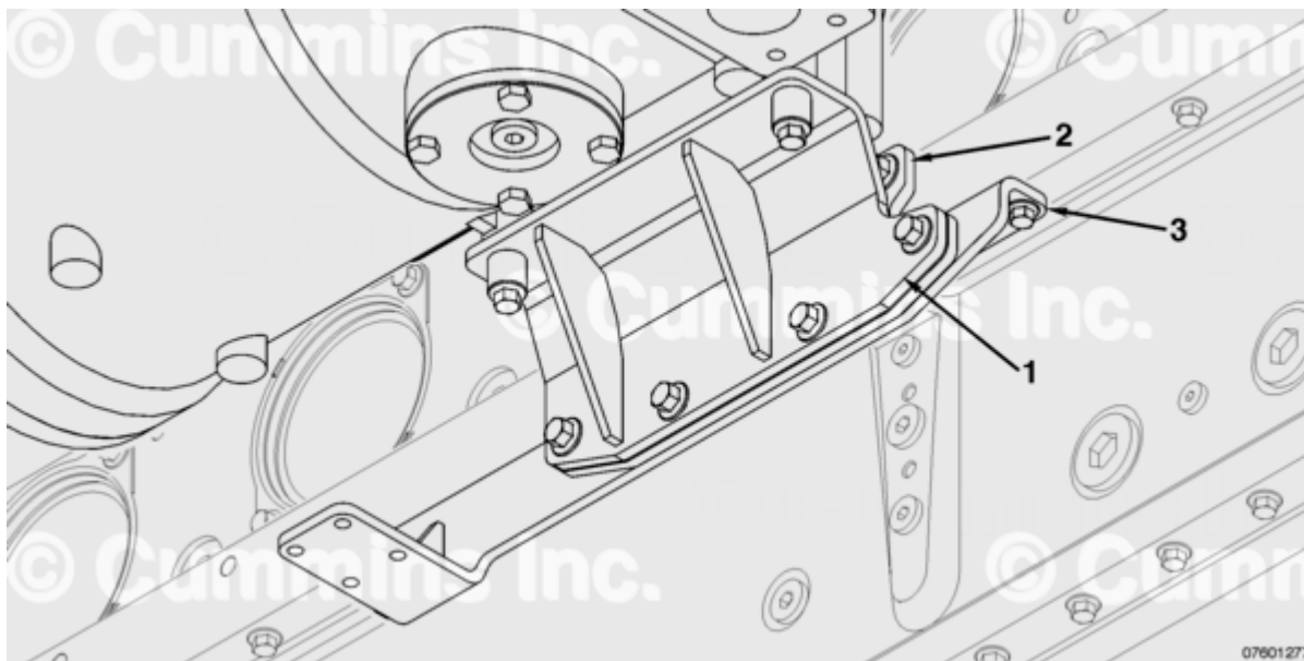
Figure 1: New Eliminator™ Support Bracket Assembly
