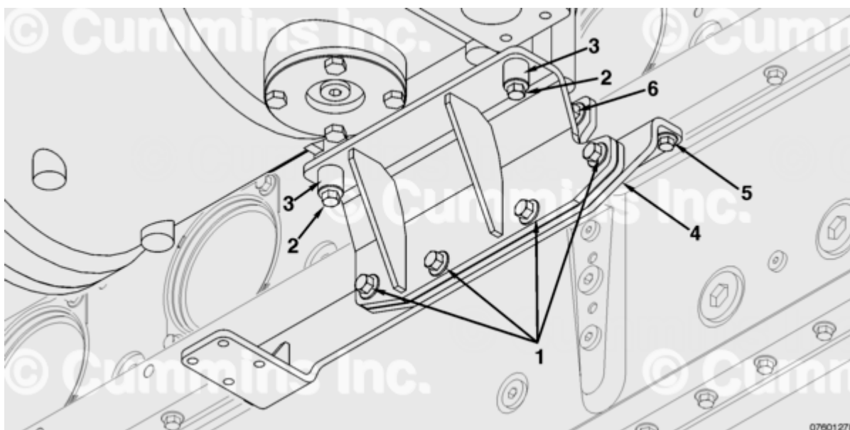
Figure 2; Mounting Components
