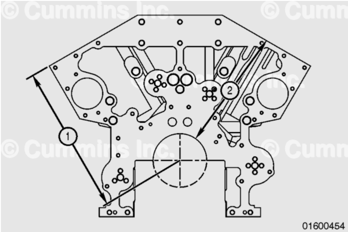
Figure 1, Block Dimension Measurement Locations
