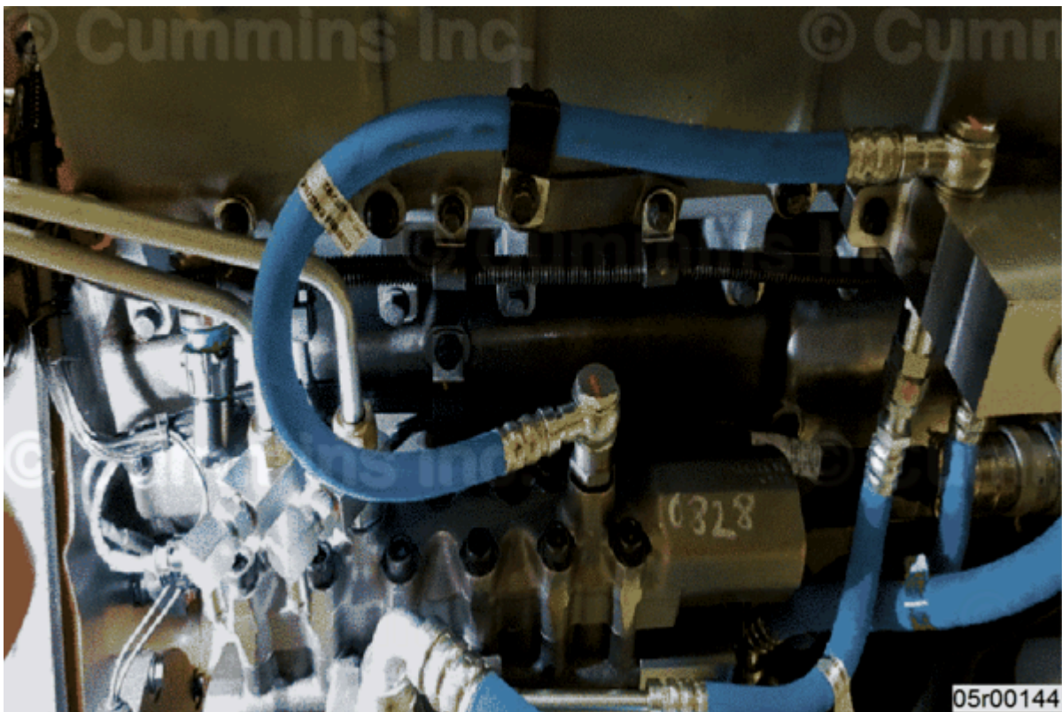
Figure 6, Using Provided Capscrews Secure Harness.
