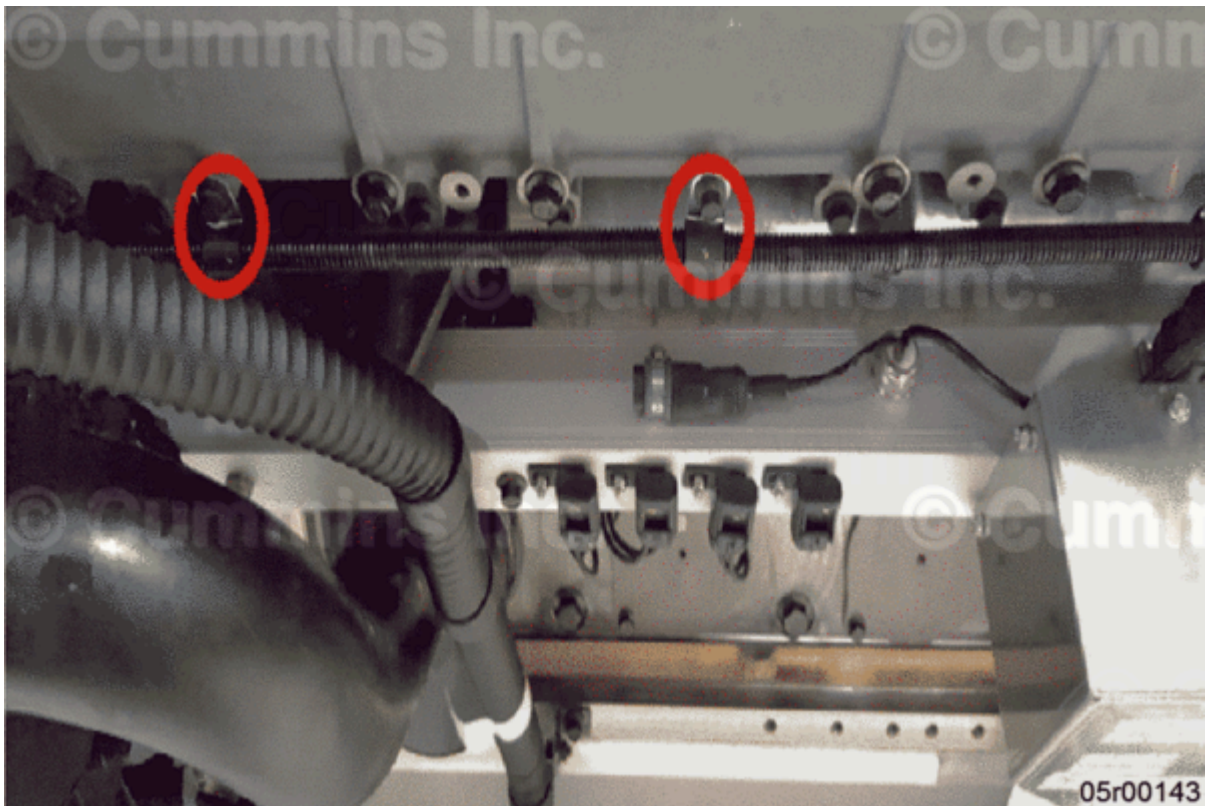
Figure 5. Use Capscrew Part Number 3093923 to Secure Harness.
