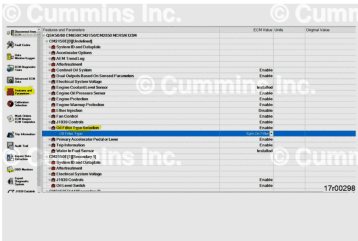
Figure 12, Lubricating Oil Filter Type Navigation.
