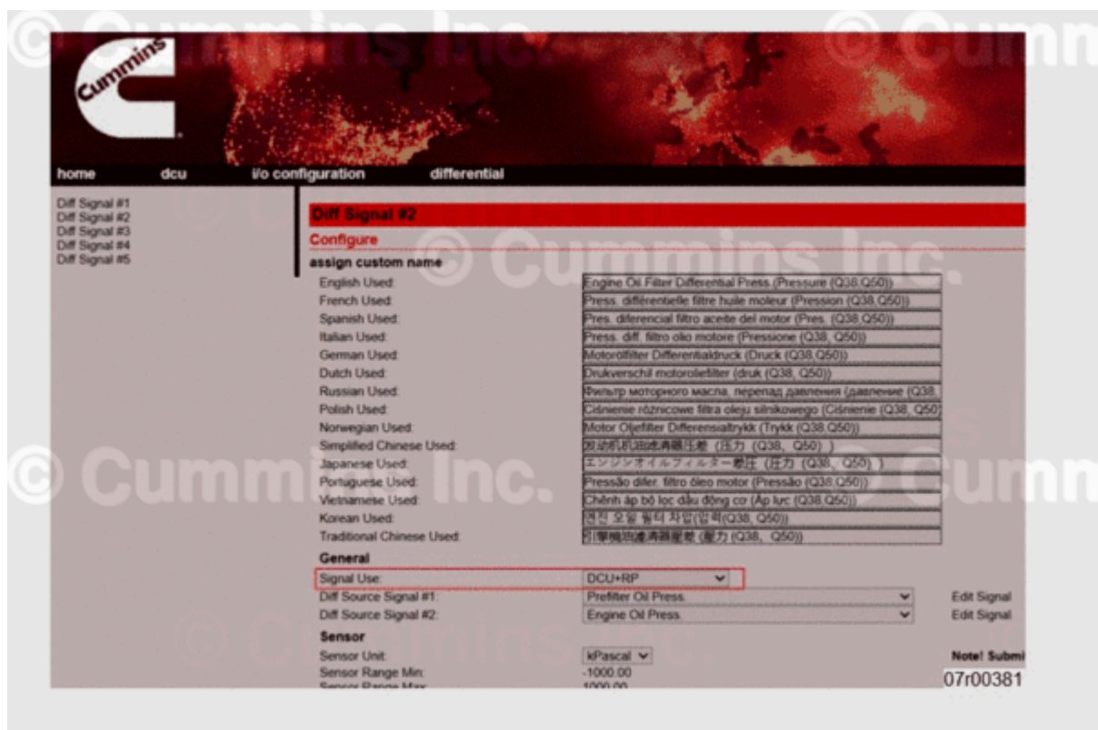
Figure 10, Diff Signal #2/#3 Screen.
