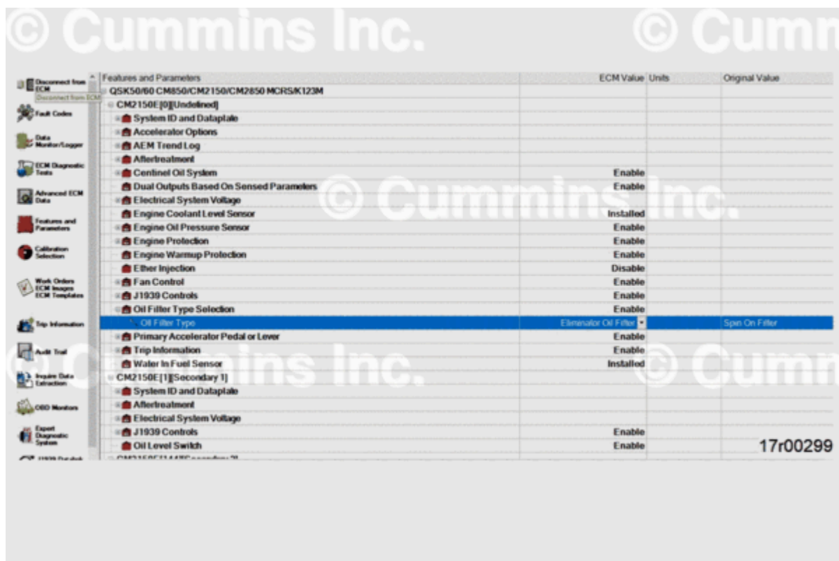
Figure 13, Select Appropriate Lubricating Oil Filter Type.
