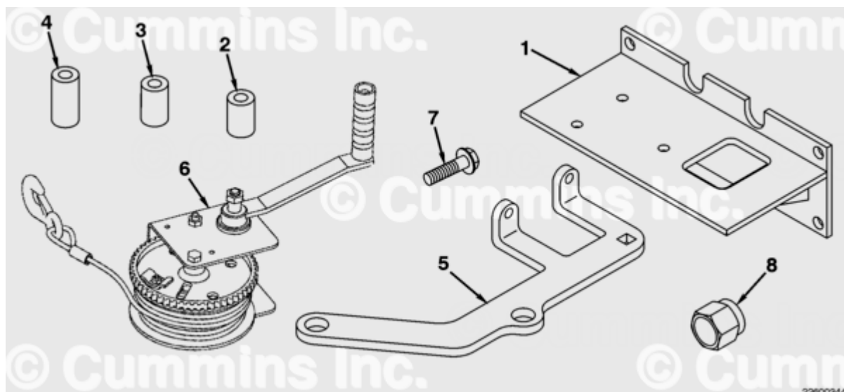
Fuel Pump Lifting Fixture Kit, Part Number 5299015
