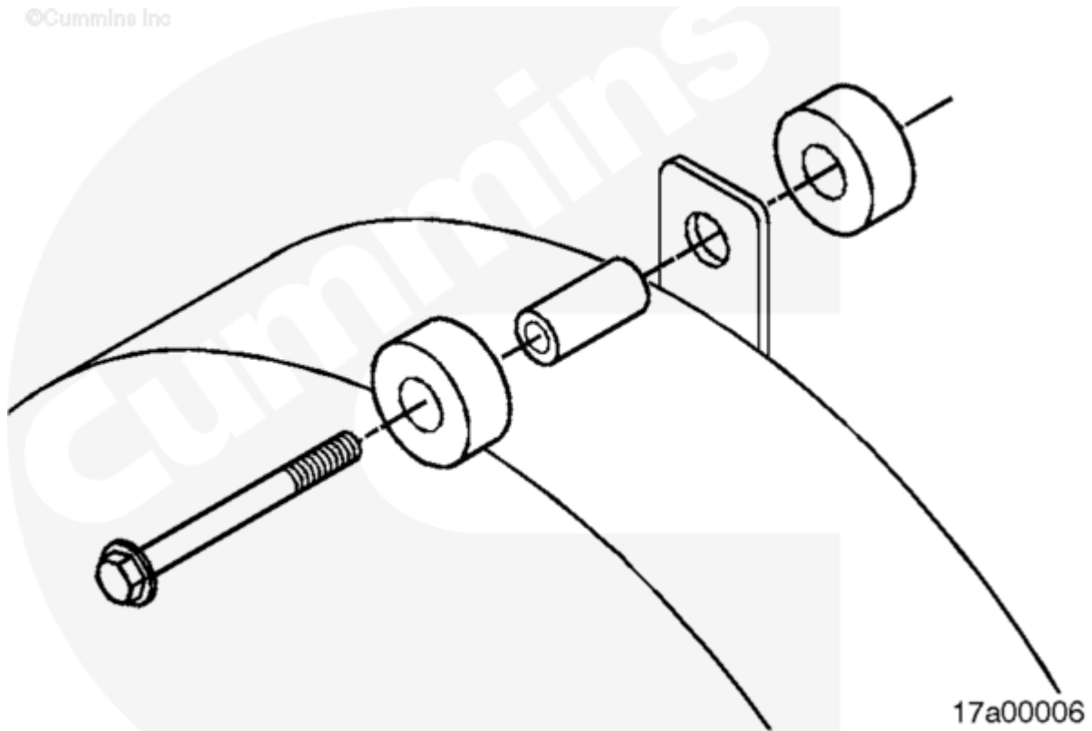
Figure 3, Spacer and Vibration Isolator Installation
