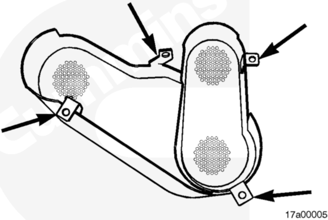
Figure 2, Belt Guard Mounting Tab Locations
