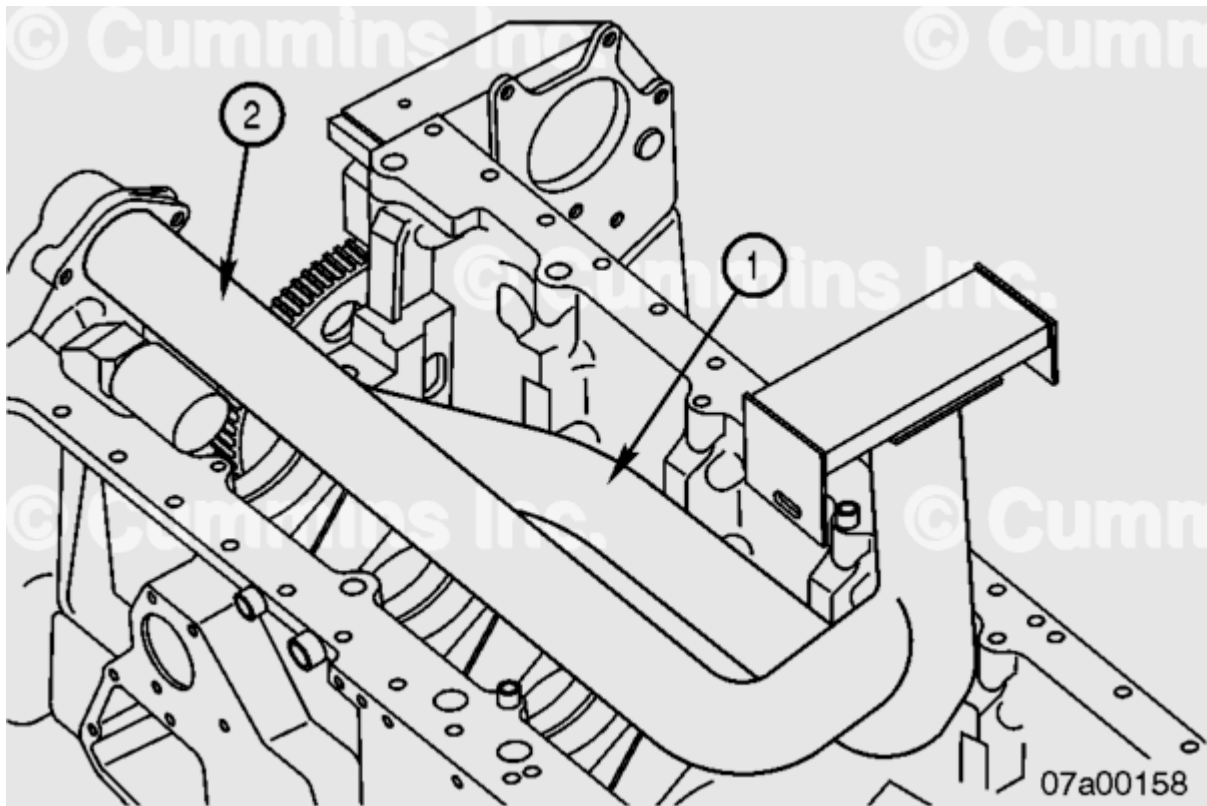
Figure 1: Bottom View - New Suction Tube (1) vs. Old Suction Tube (2)
