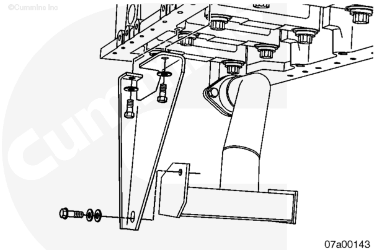
Figure 2: Obsolete Side-Mount Bracket
