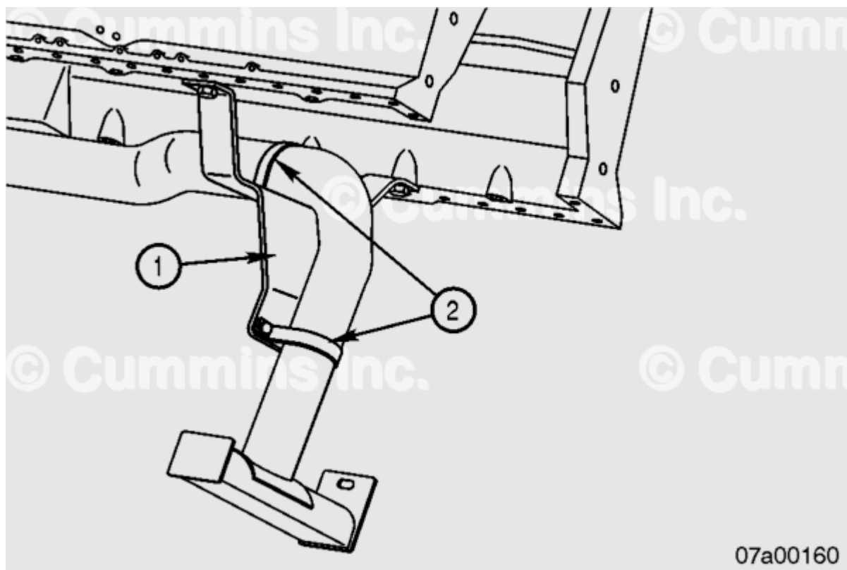
Figure 3: New Center-Mount Bracket (1) and Clamps(2)
