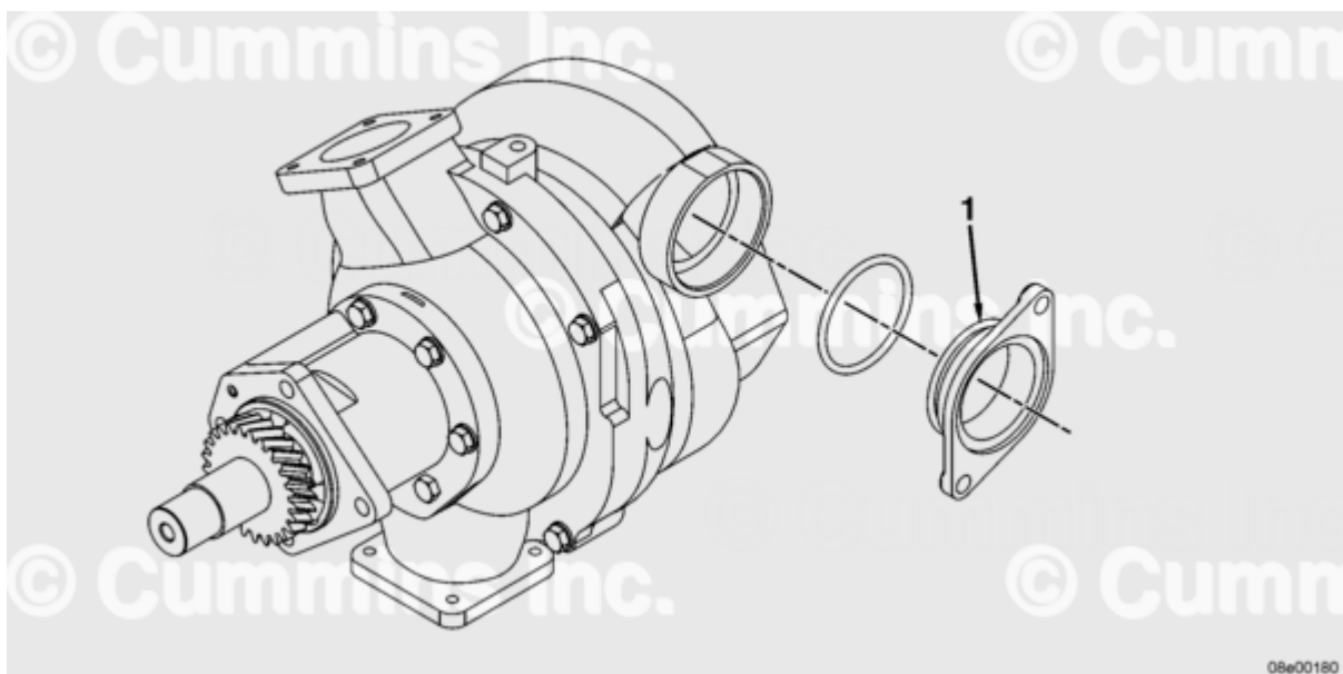
New O-ring Adapter, Part Number 3644172
