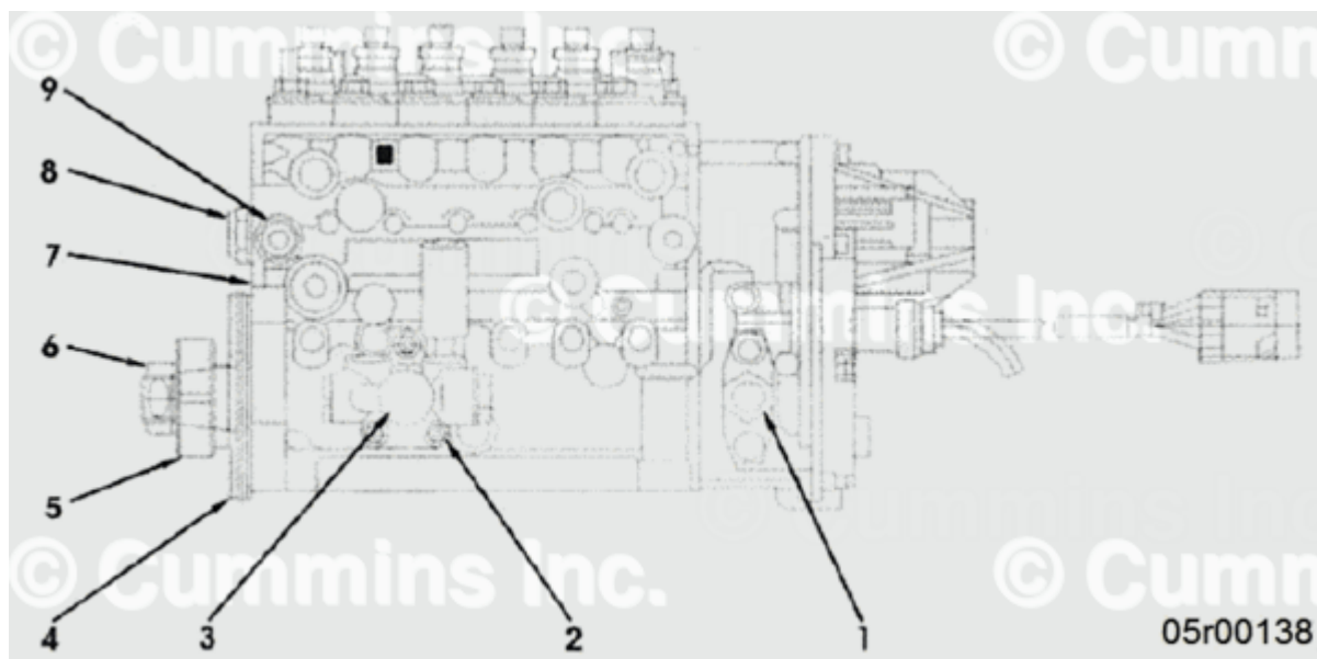
Figure 3, Generator-Drive Flange Mount Fuel Pump.
