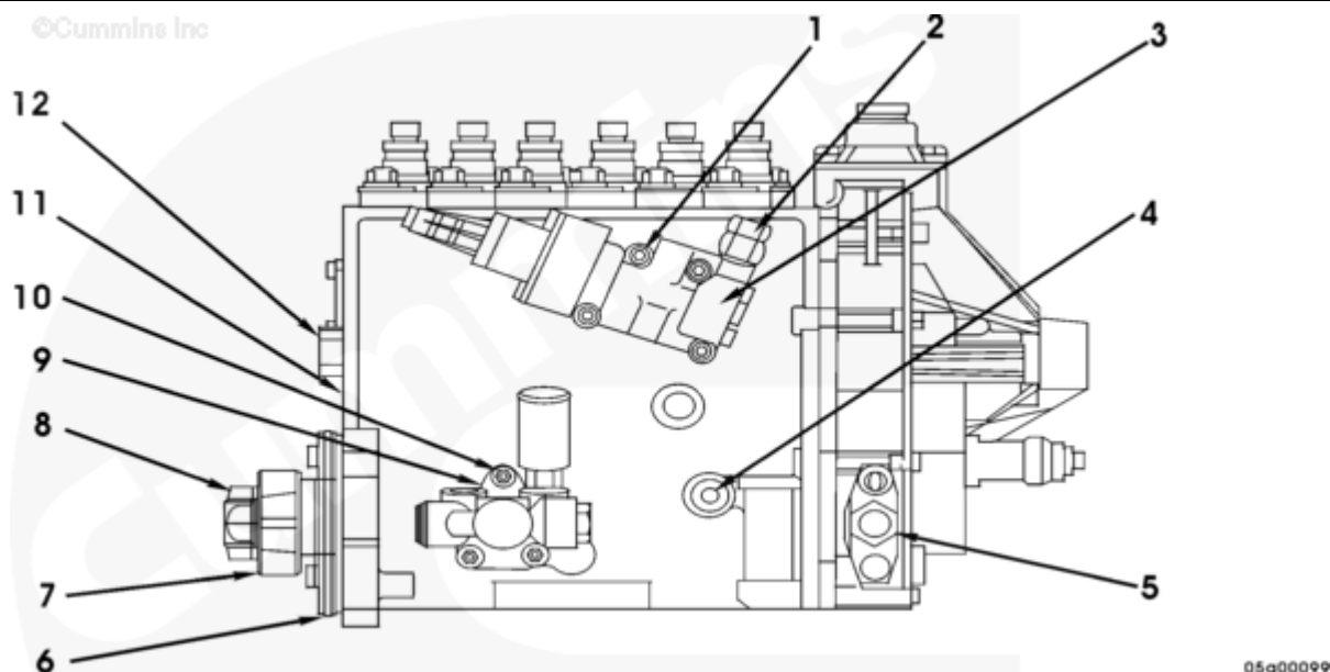
Figure 2, Industrial Fuel Pump (RP39).
