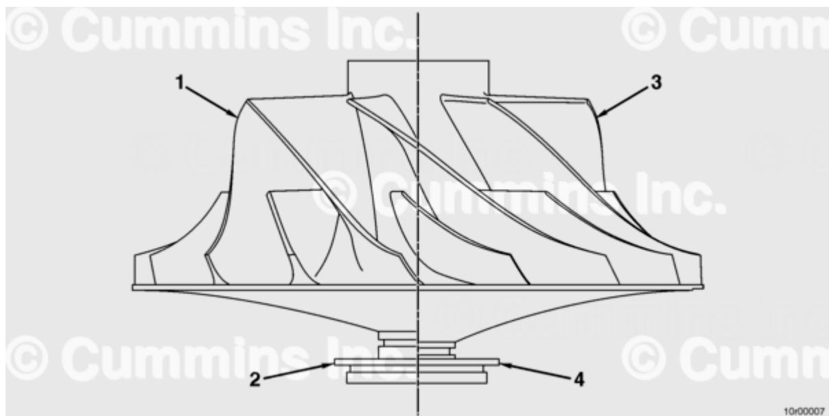
Figure 2; Comparison of Old Impeller Wheel (1) / Oil Slinger (2) and New Impeller Wheel (3) / Oil Slinger (4).
