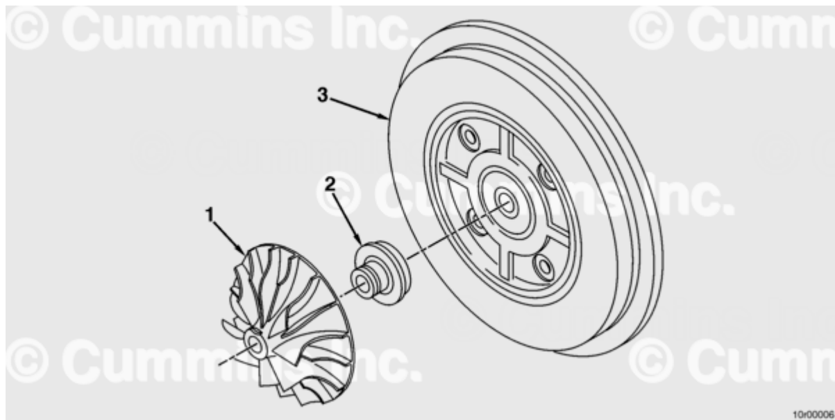
Figure 1; Parts affected in the impeller supersession: Impeller (1), Oil Slinger (2), and Diffuser (3).
