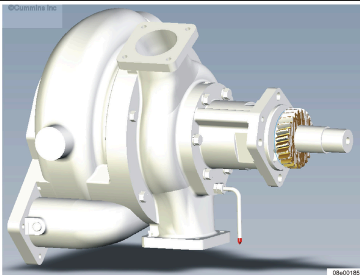
Figure 1, New water pump with weep hole relocated and filter installed.
