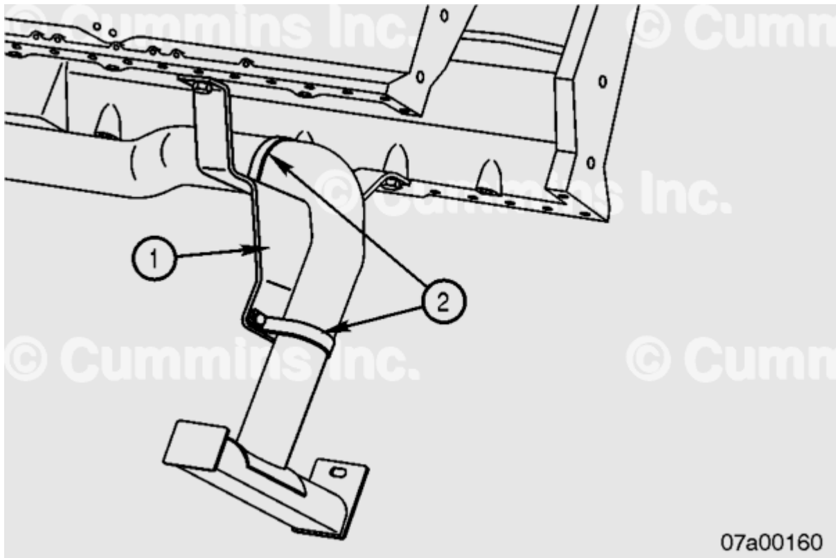
Figure 1: Obsolete Center-Mount Bracket (1) and Clamps (2)
