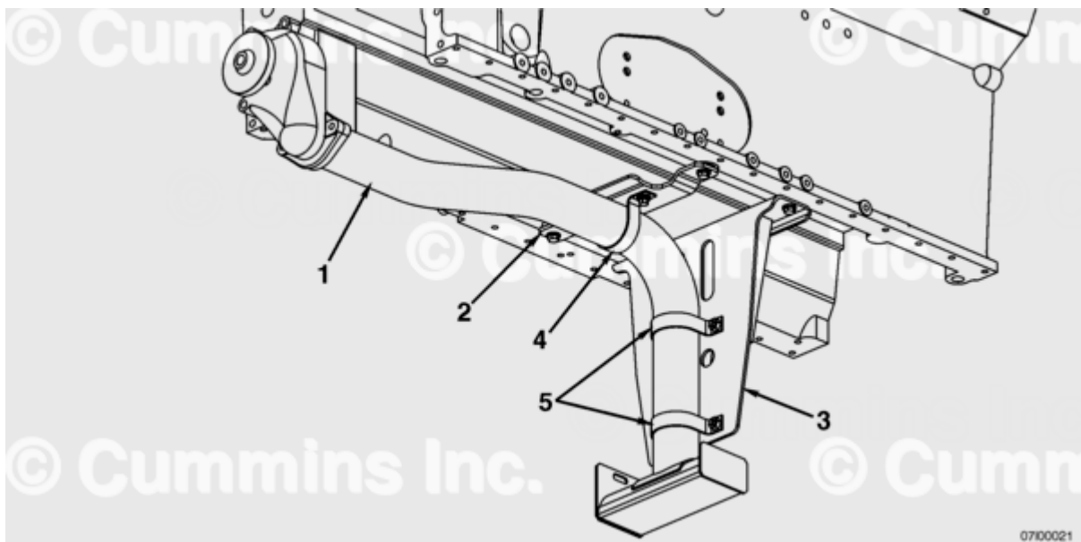
Figure 2: New Suction Tube (1), Block Bracket (2), Vertical Bracket (3), Block Bracket Tube Clamp (4), and Tube Clamp (5)
