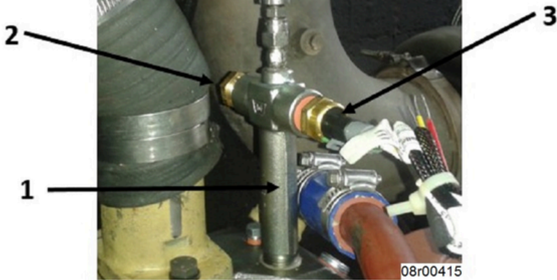
Figure 1, Coolant Tee Adapter with Engine Coolant Temperature Sensor and Engine Coolant Temperature Switch
