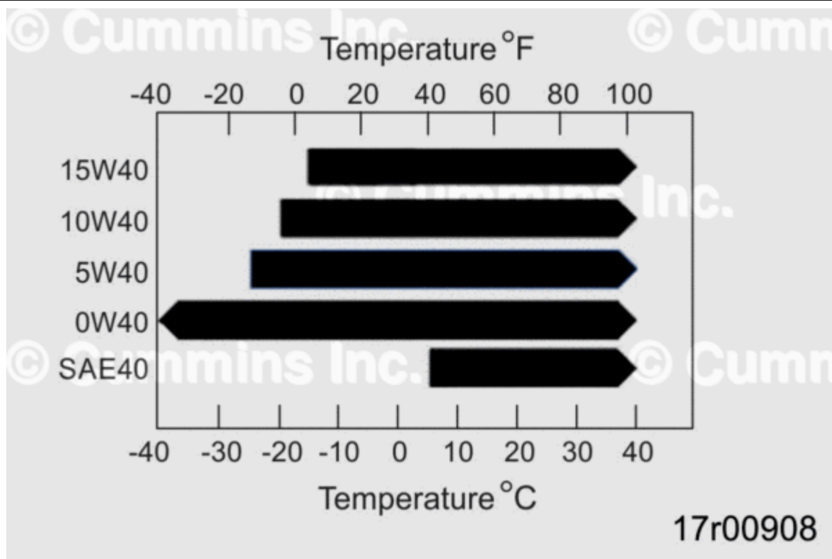
Figure 1, Recommended SAE Oil Viscosity Grades vs Ambient Temperatures
