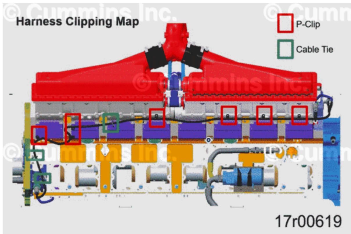
Figure 6, Secure Wire Harness
