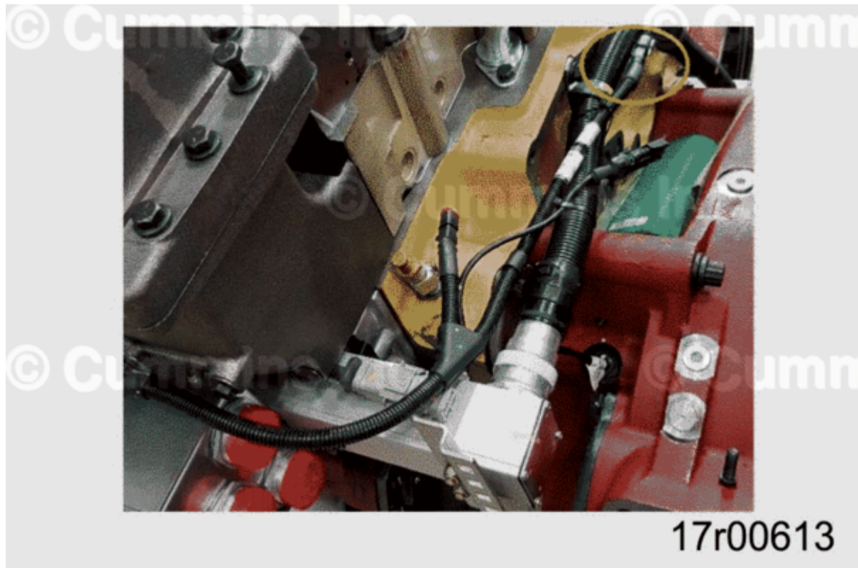
Figure 2, Pressure Switch Wire Harness Extension
