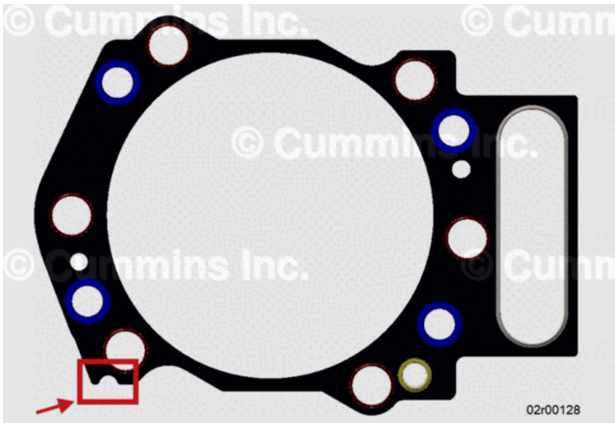
Figure 1, Existing Oversized Cylinder Head Gasket Design Showing Notch at Bottom Left (For Differentiation Purposes Only).
