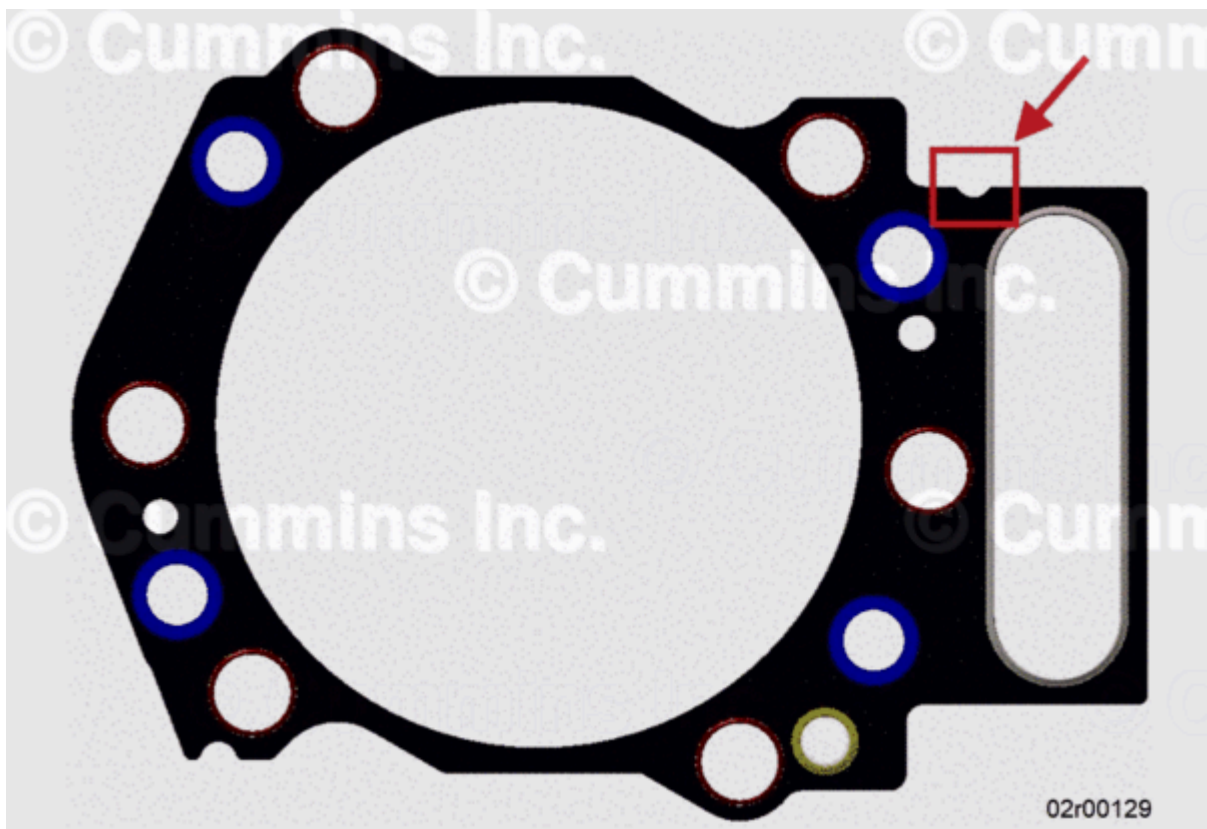
Figure 2, New 0.25 mm Oversized Cylinder Head Gasket Showing One Notch at Upper Right.
