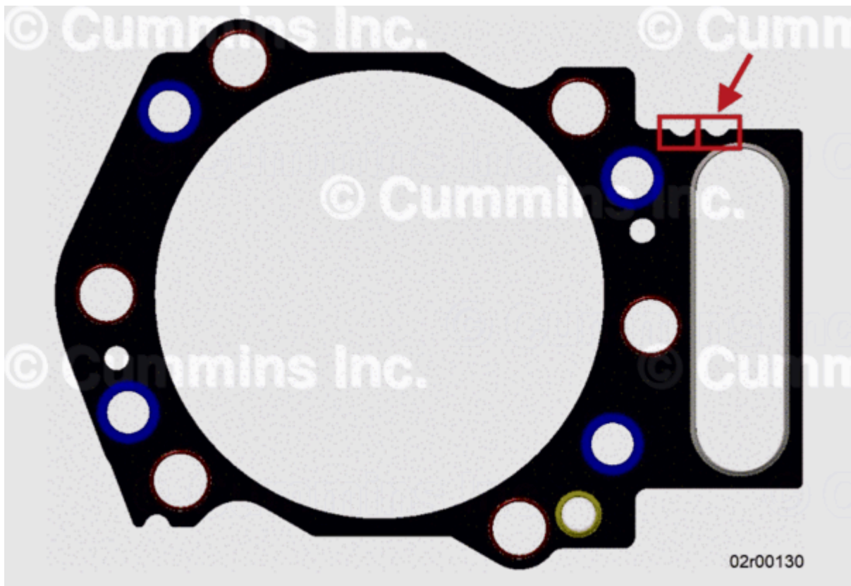
Figure 3, New 0.5 mm Oversized Cylinder Head Gasket Showing Two Notches at Upper Right.
