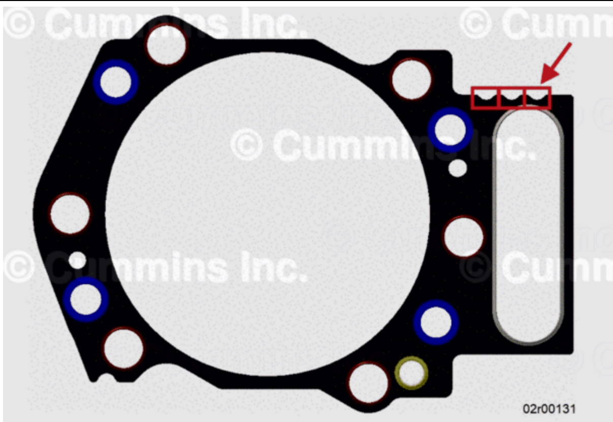
Figure 4, New 0.75 mm Oversized Cylinder Head Gasket Showing Three Notches at Upper Right.
