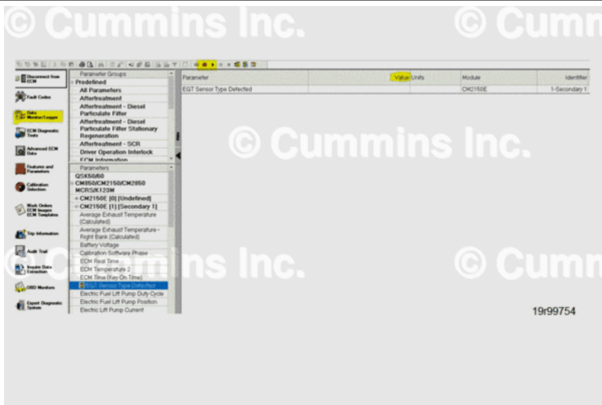
Figure 8, Monitoring EGT Sensor Type Detected.
