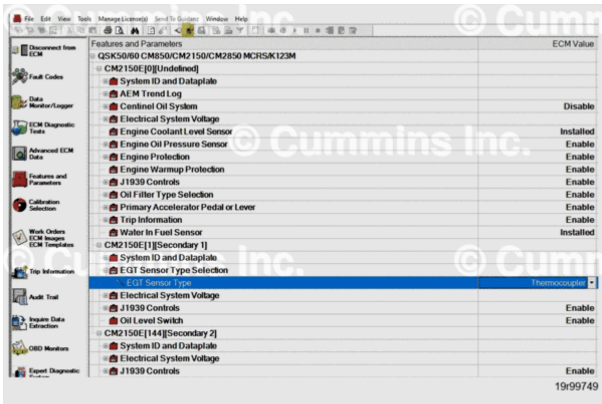
Figure 3, Select "Send to ECM".
