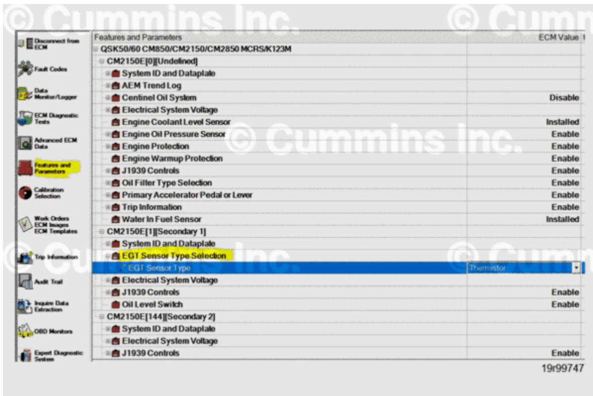
Figure 1, EGT Sensor Type Navigation.
