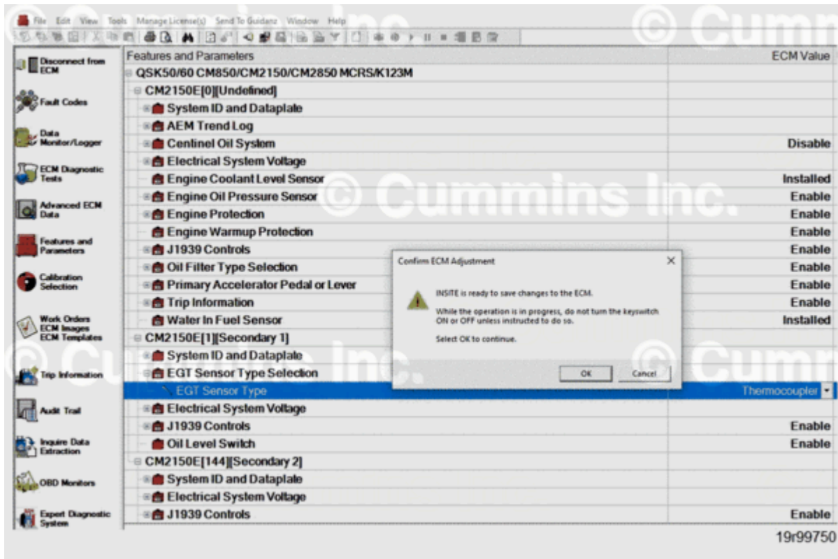
Figure 4, Confirm ECM Adjustment.
