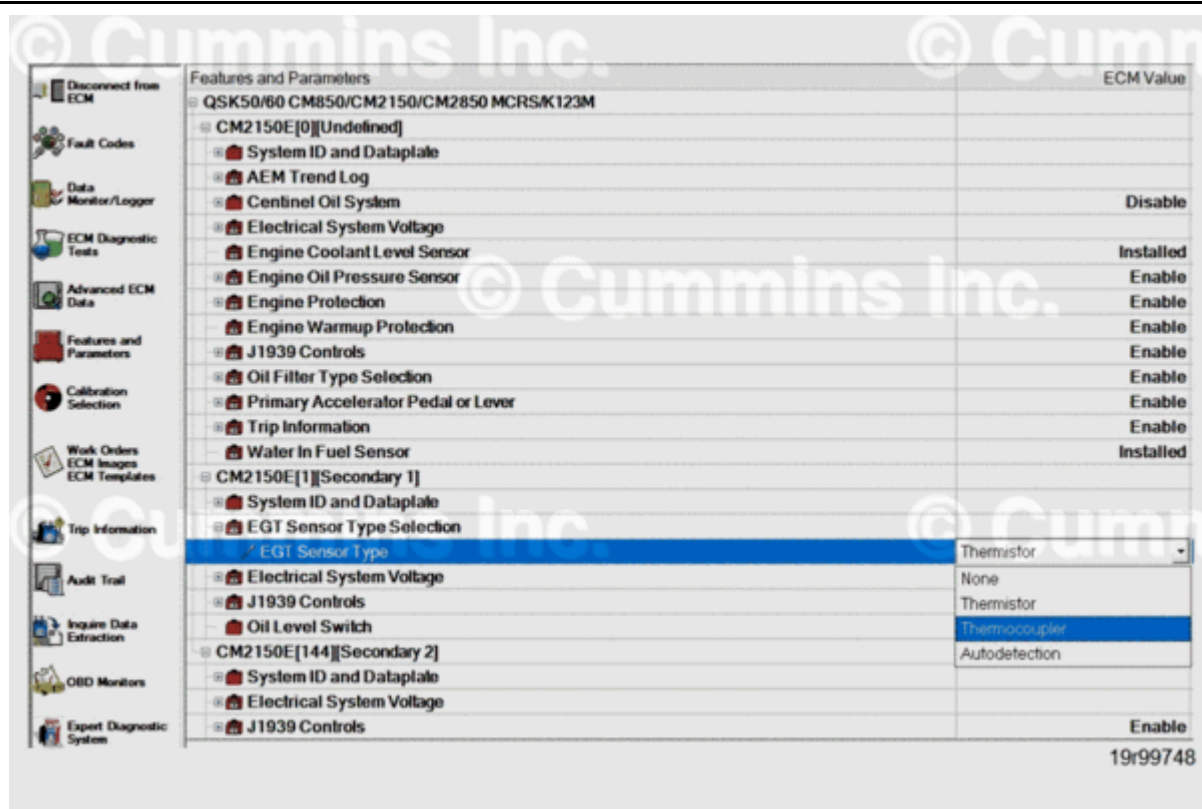
Figure 2, Select Appropriate EGT Sensor Type.
