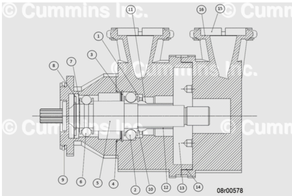
Figure 1, LTA Water Pump.
