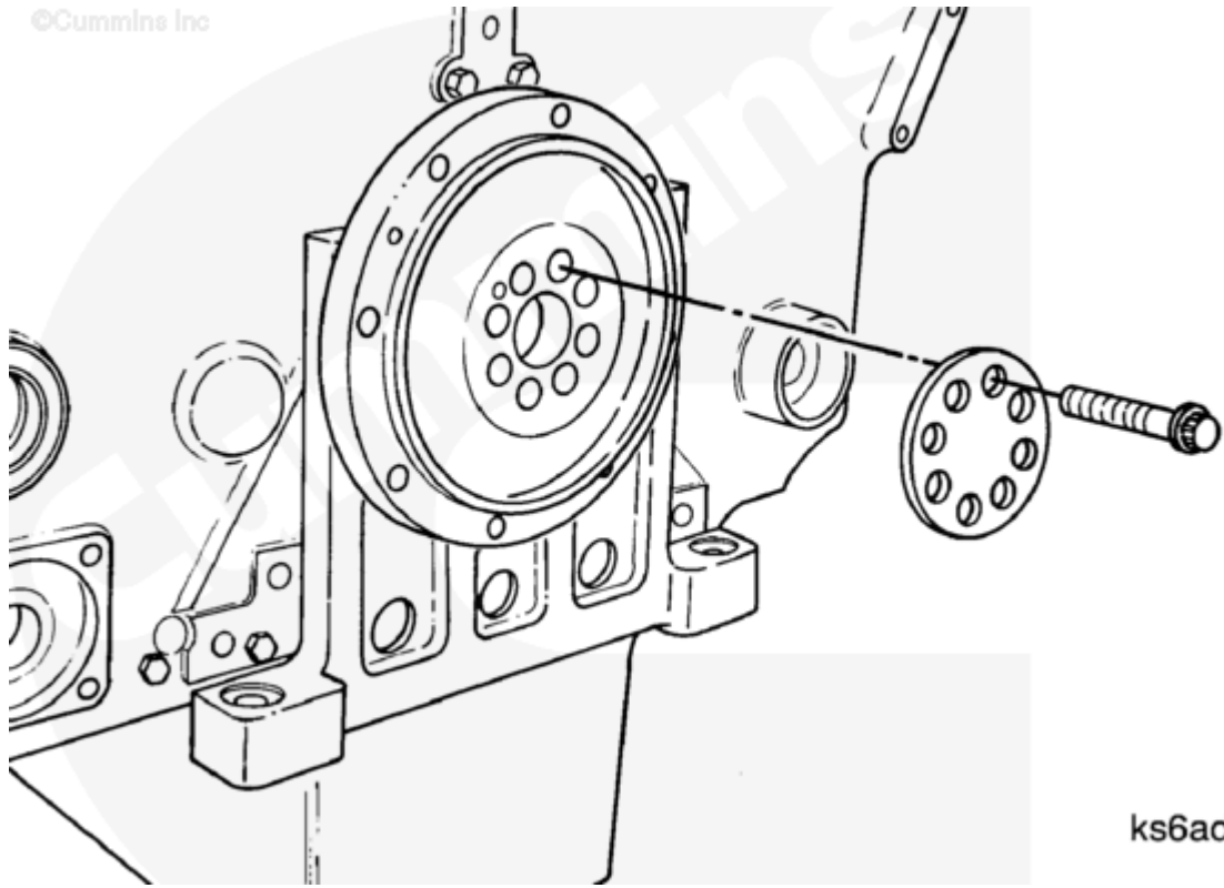
Figure 1, Crankshaft Adapter Capscrews.
