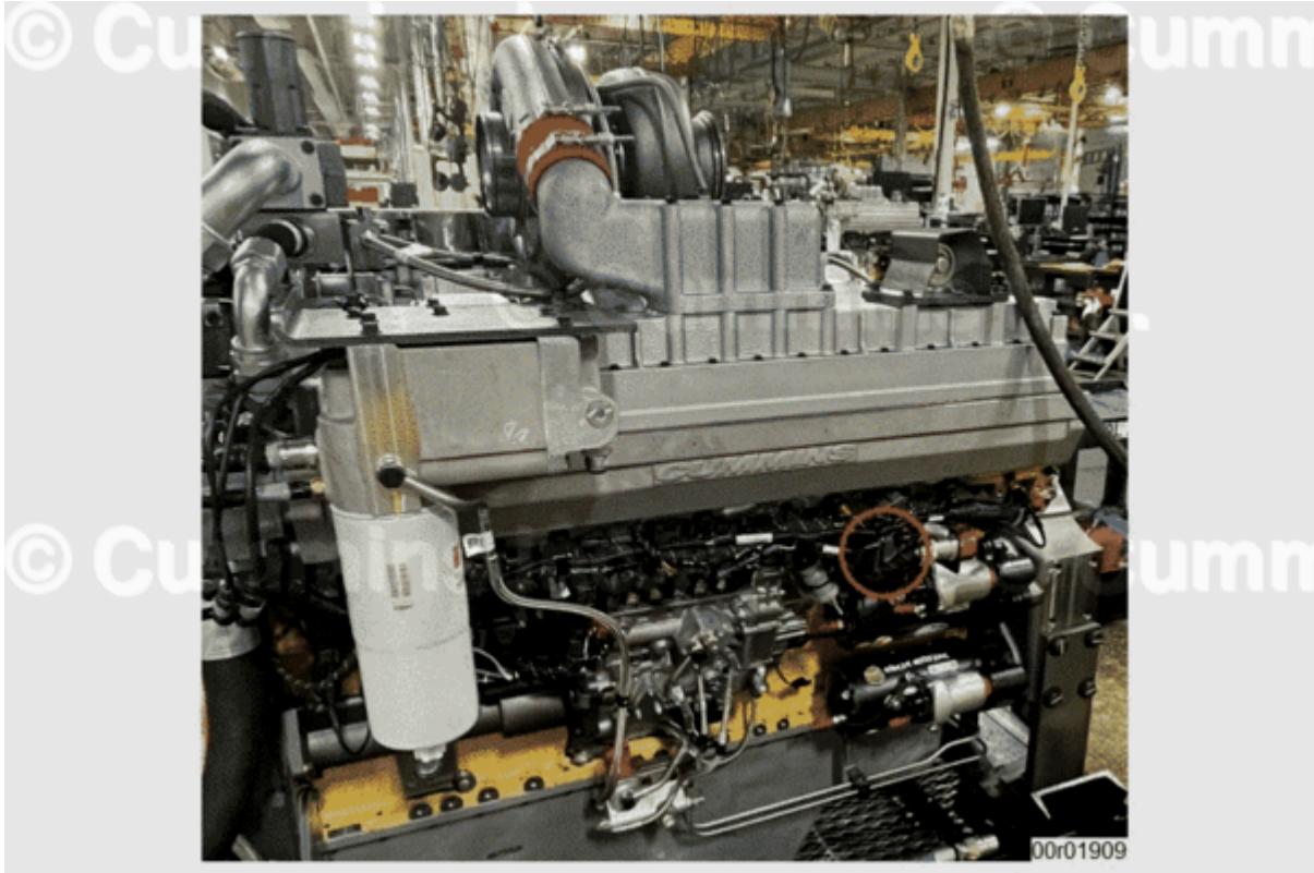
Figure 1, Engine Left Bank Fuel Lift Pump Relay Location.
