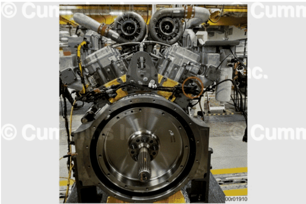
Figure 2, Engine Rear Fuel Lift Pump Relay Location.
