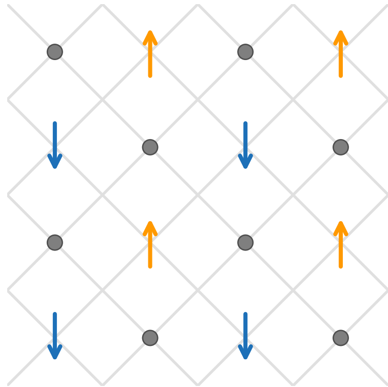
Altermagnet
