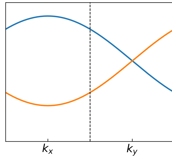
Altermagnet
