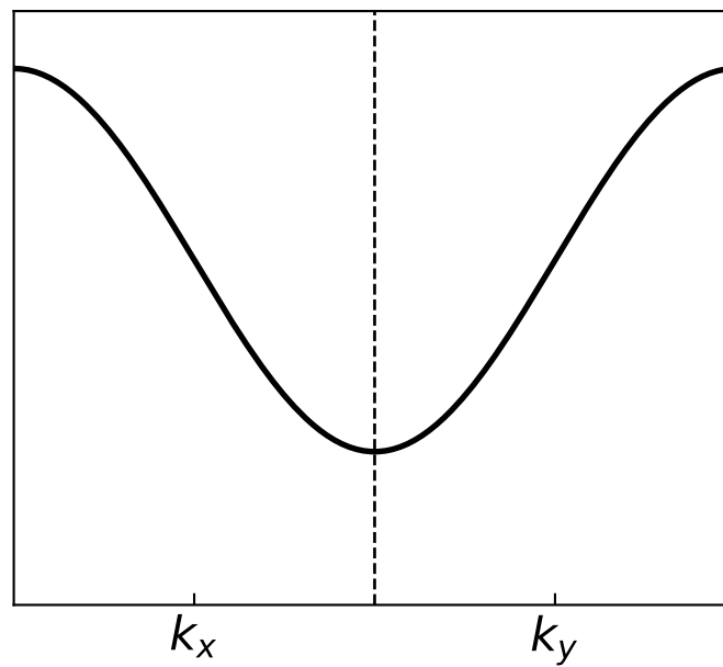
Antiferromagnet
