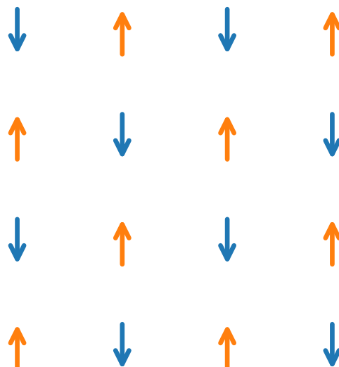
Antiferromagnet
