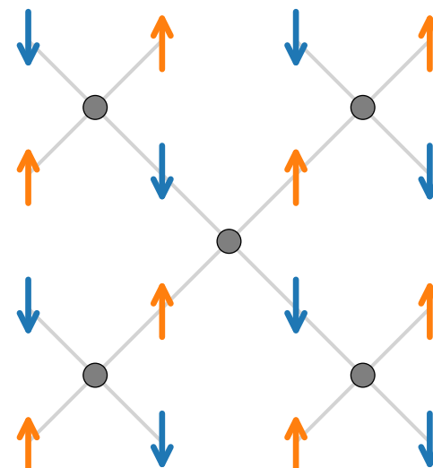
Altermagnet
