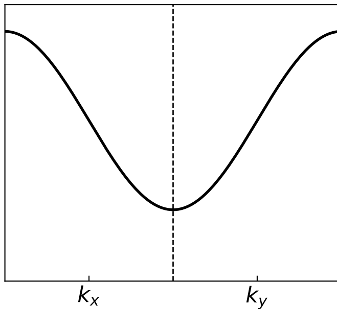
Antiferromagnet
