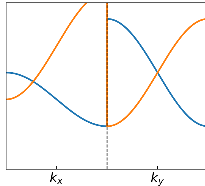
Altermagnet
