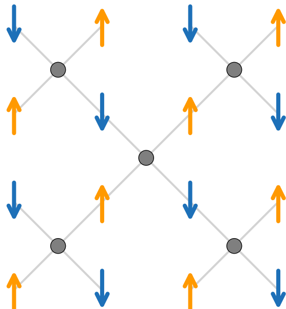
Altermagnet
