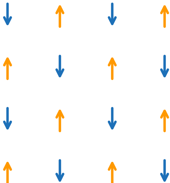
Antiferromagnet
