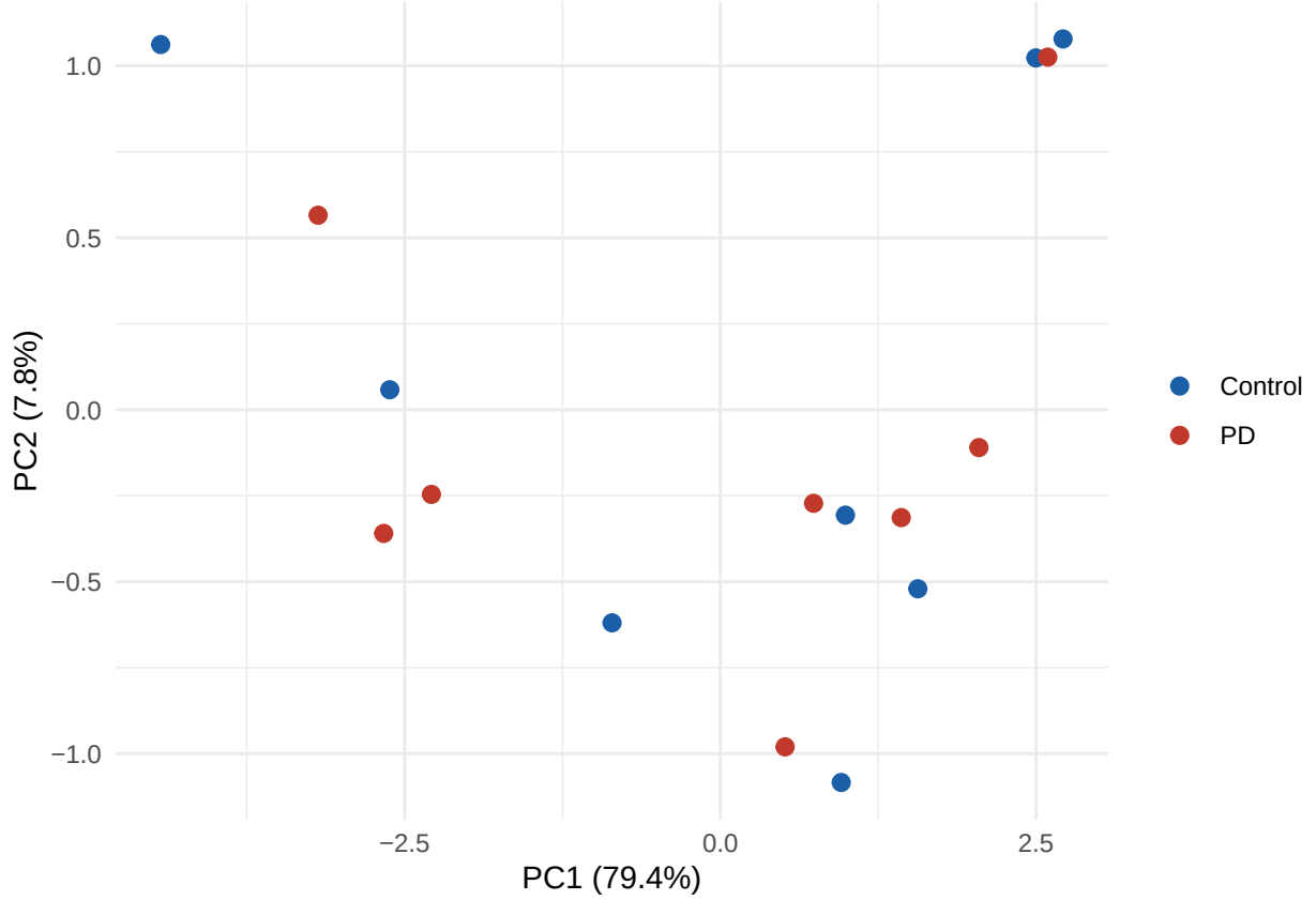
Figure 4: FPC scores, native space, H_2 , main definition. No grouping structure is visible.
