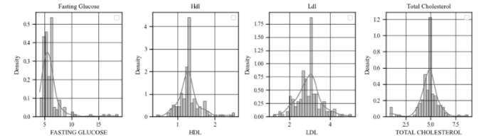
Figure 4. Distributions of FPG, HDL, LDL, and Total Cholesterol - manic subset
