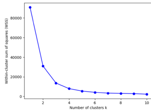
Figure 9: Elbow Method for Optimal K
