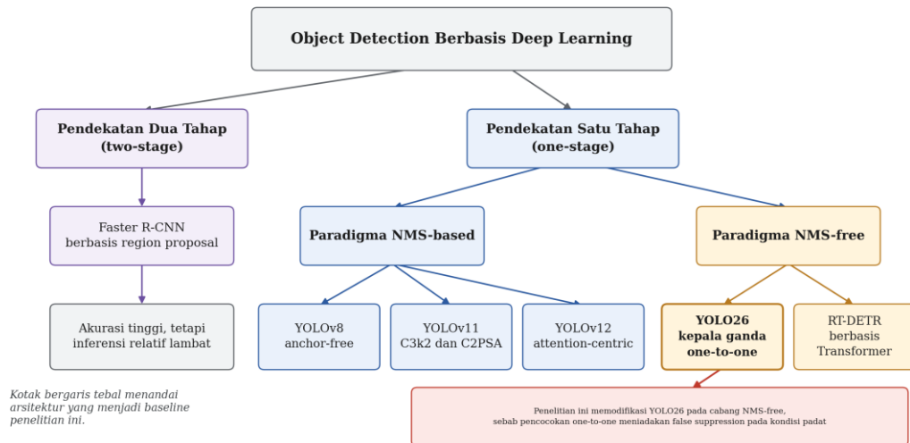
Gambar 2.1 Taksonomi Metode Object Detection Berbasis Deep Learning
