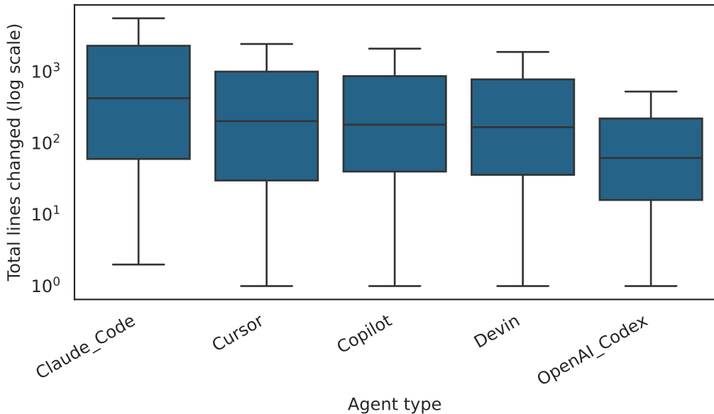
Code diff size by agent type
