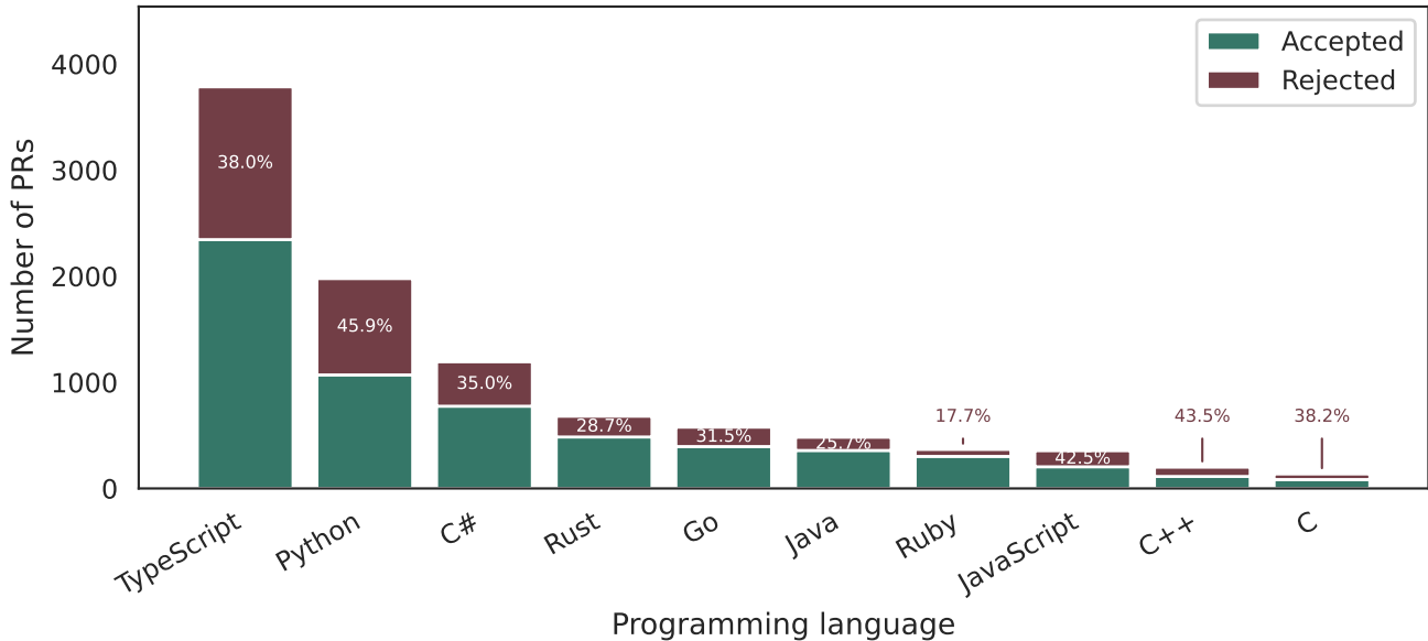
PR count by programming language (top 10)
