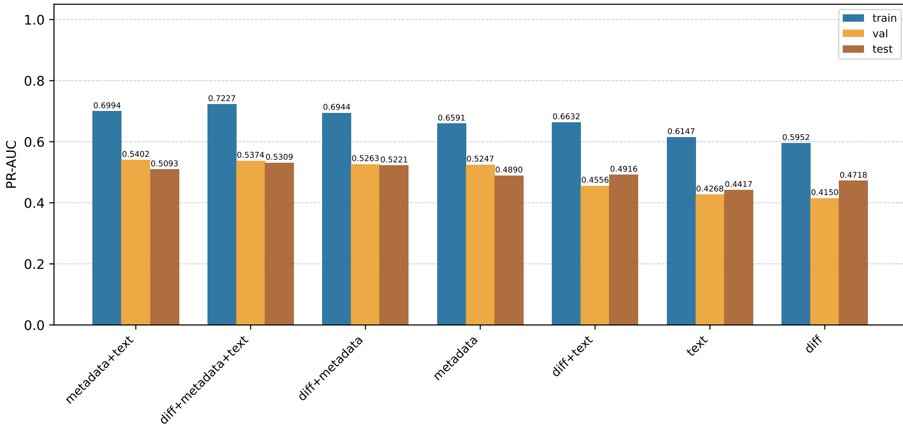
Multimodal Logistic Regression Group Ablation
