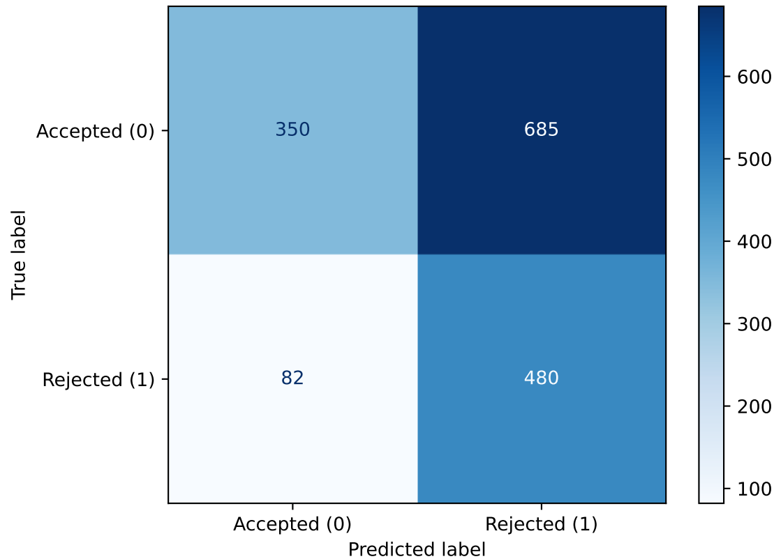
Confusion Matrix
