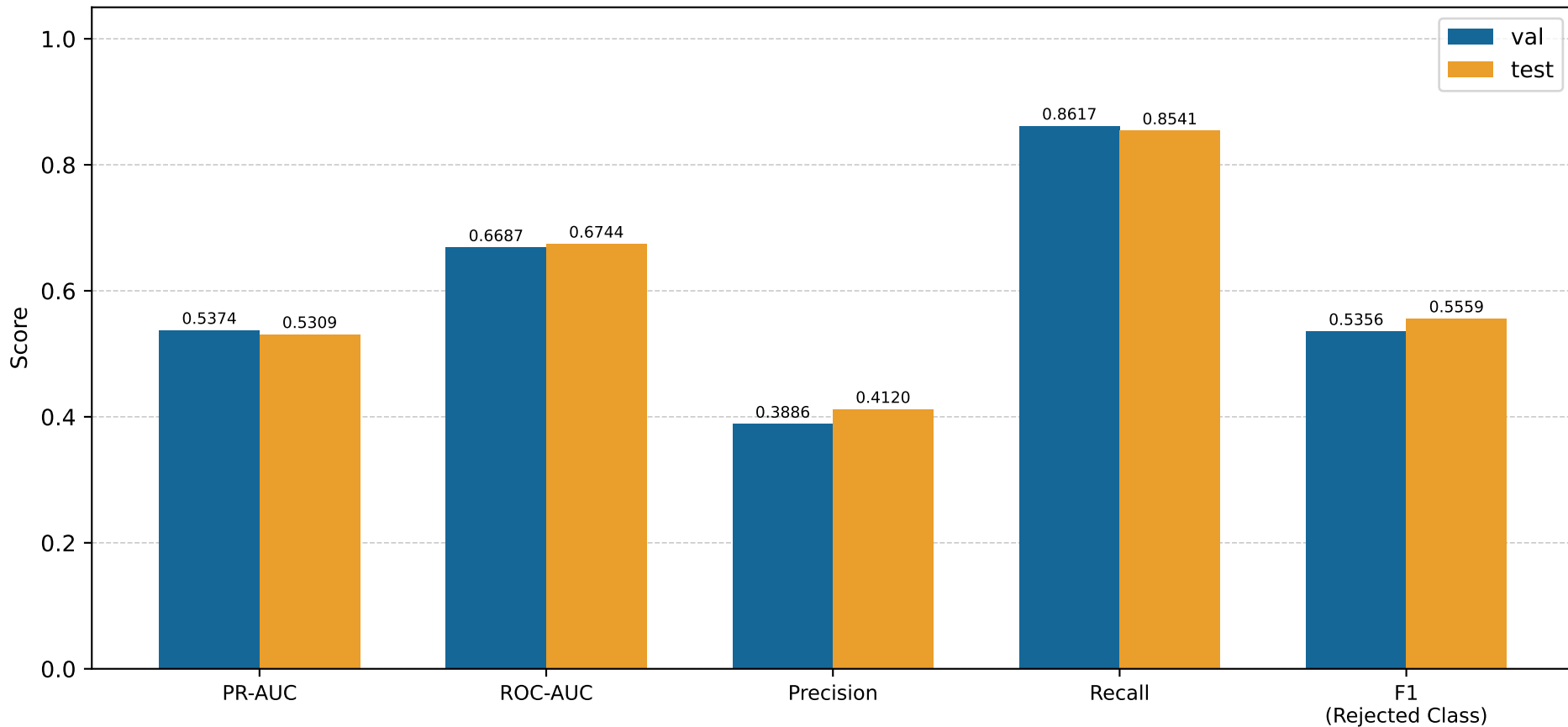
Metric Comparison — Multimodal Logistic Regression (Val vs Test)
