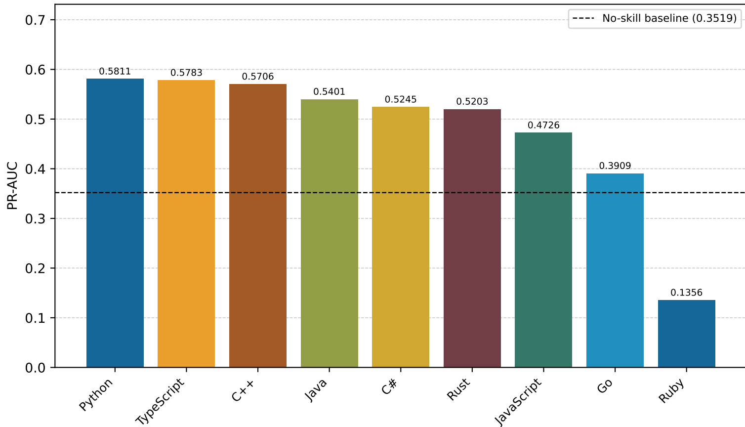
Multimodal Logistic Regression PR-AUC by language — Test
