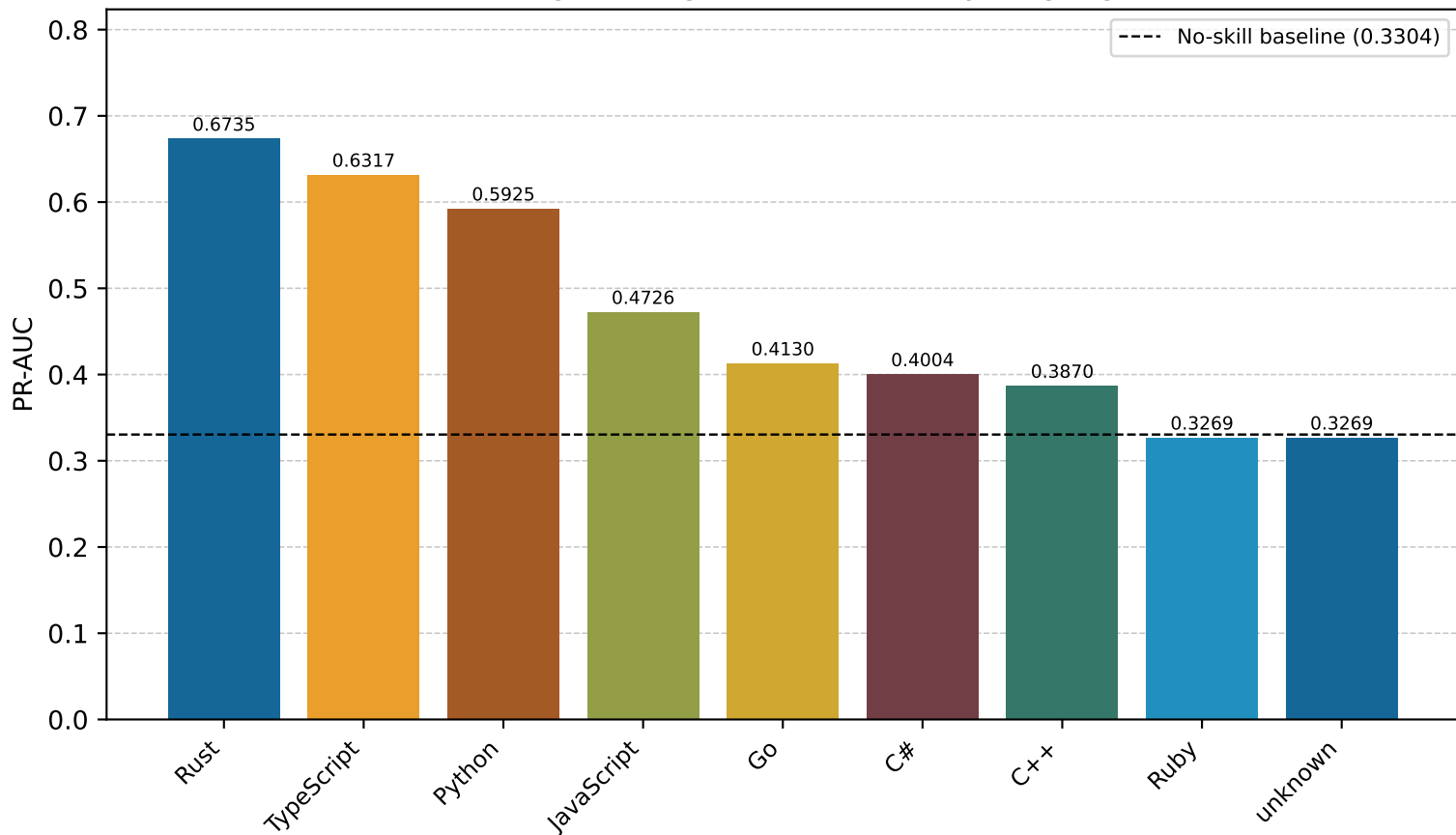
Multimodal Logistic Regression PR-AUC by language — Val
