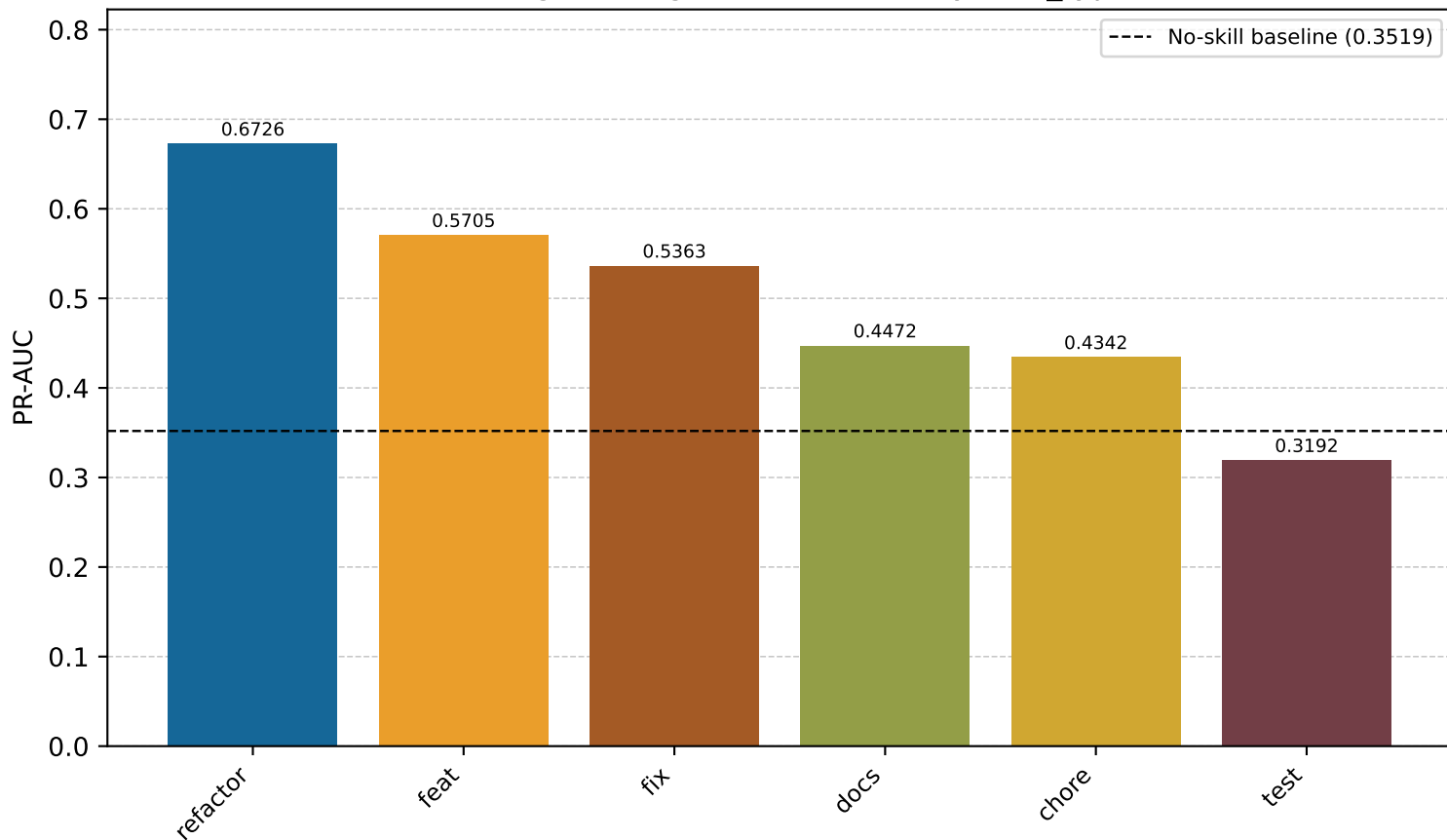
Multimodal Logistic Regression PR-AUC by task_type — Test
