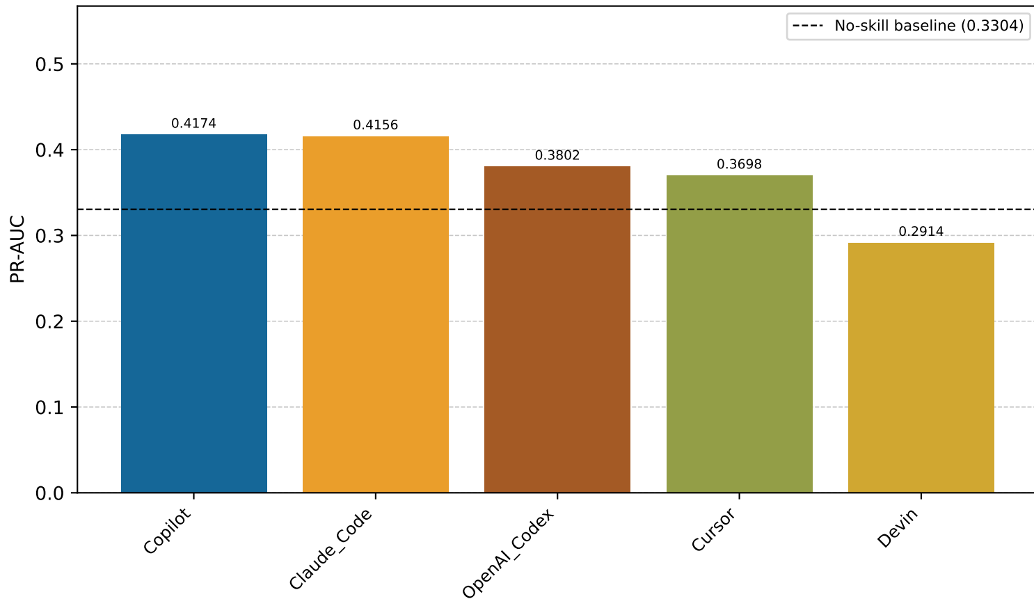
Qwen3 Standard LLM PR-AUC by agent — Val
