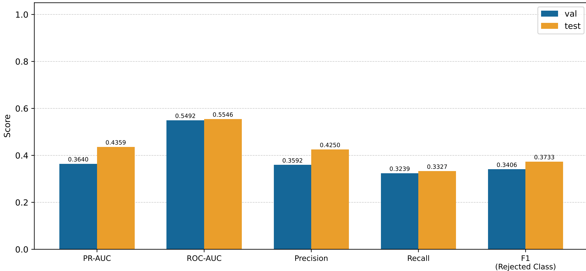
Metric Comparison — QwQ Reasoning LLM (Val vs Test)
