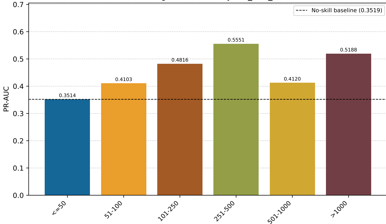
QwQ Reasoning LLM PR-AUC by diff_size_bin — Test
