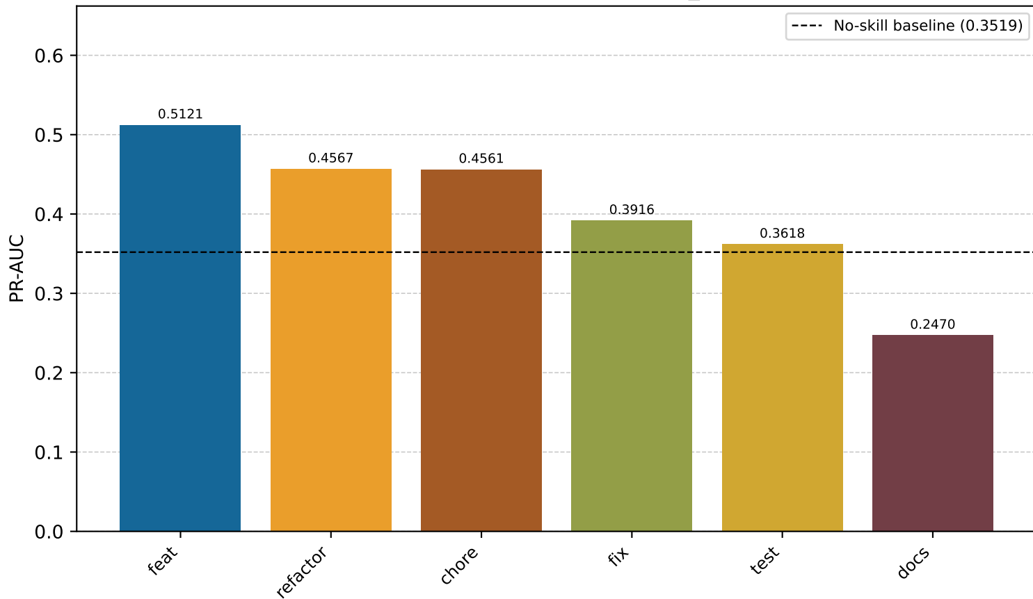
QwQ Reasoning LLM PR-AUC by task_type — Test
