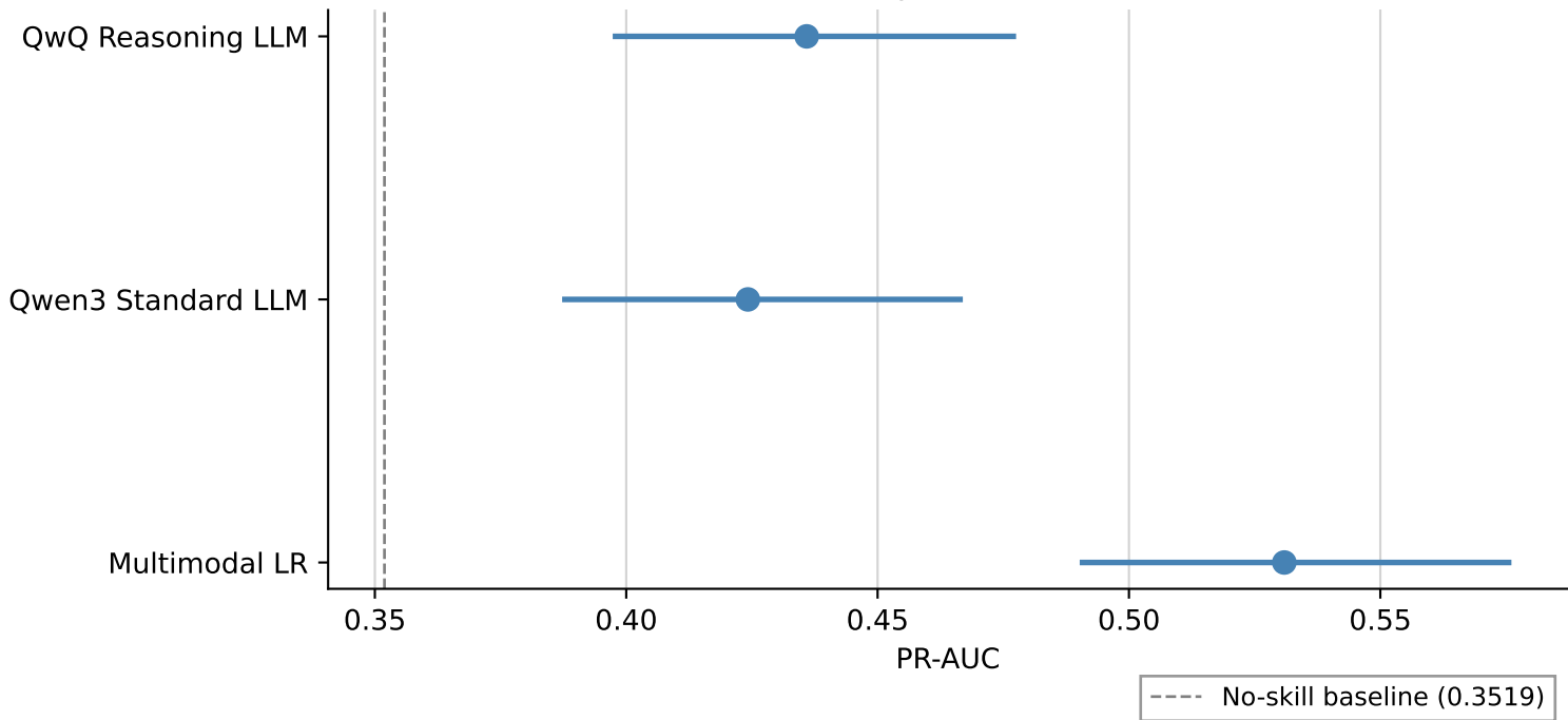
PR-AUC with 95% Bootstrap Confidence Intervals (Test Set)
