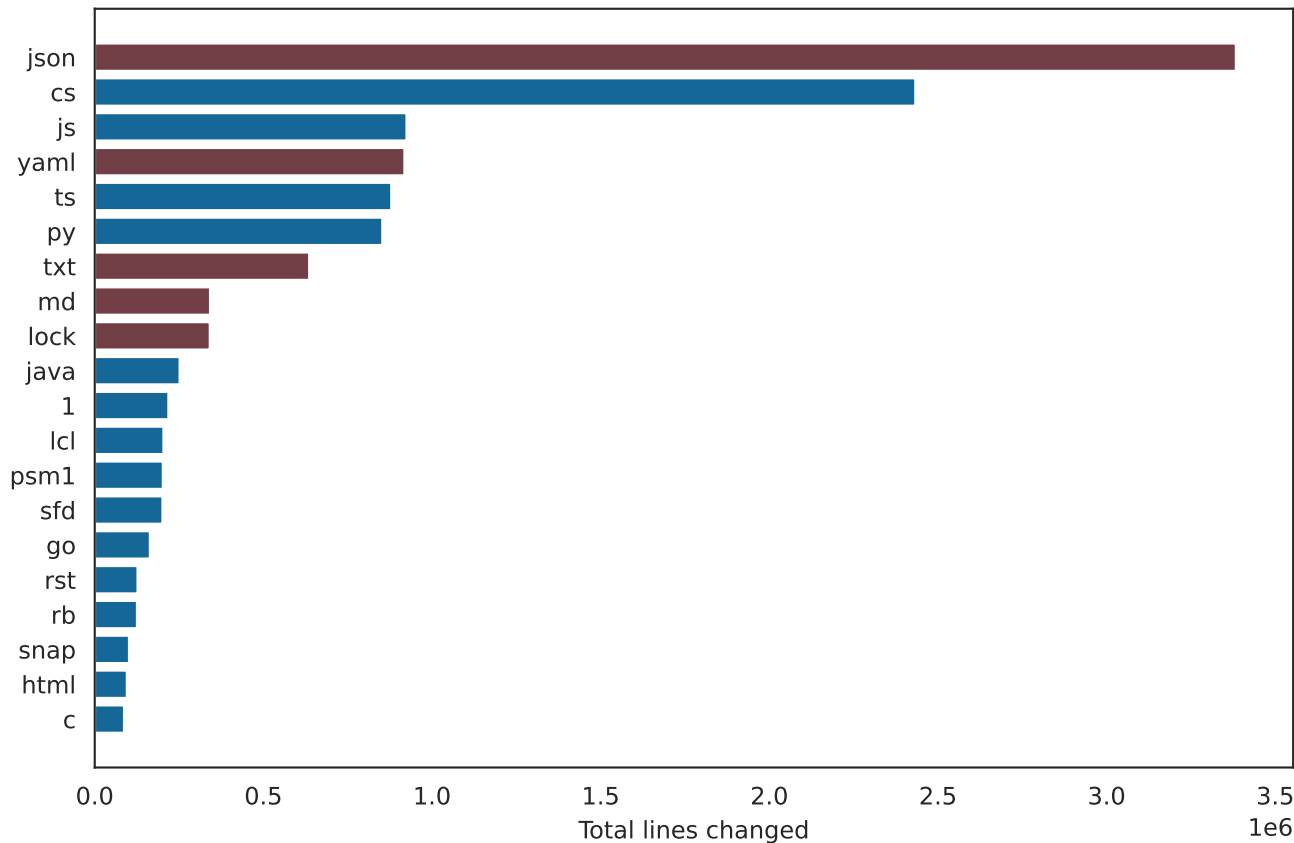
File extensions in outlier PRs (above 50,000 lines) Dark maroon = likely non-semantic file type
