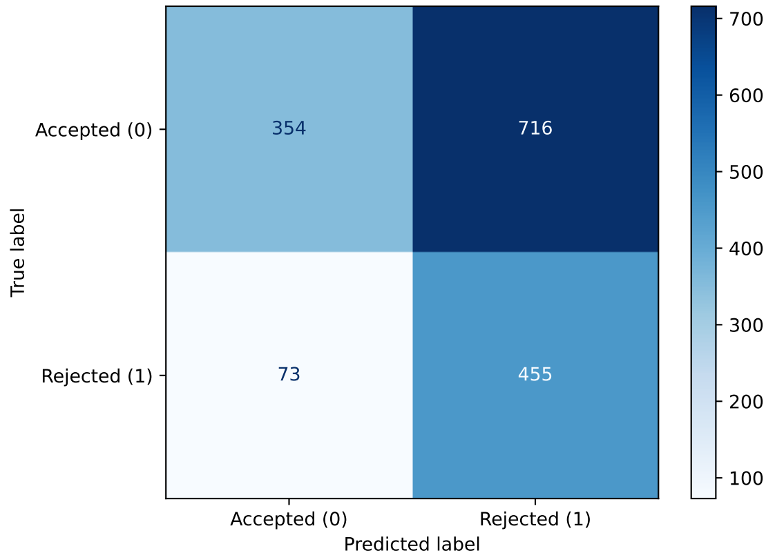
Confusion Matrix
