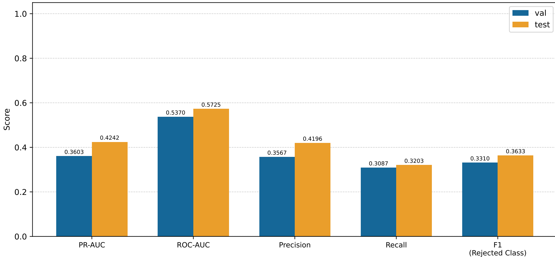
Metric Comparison — Qwen3 Standard LLM (Val vs Test)
