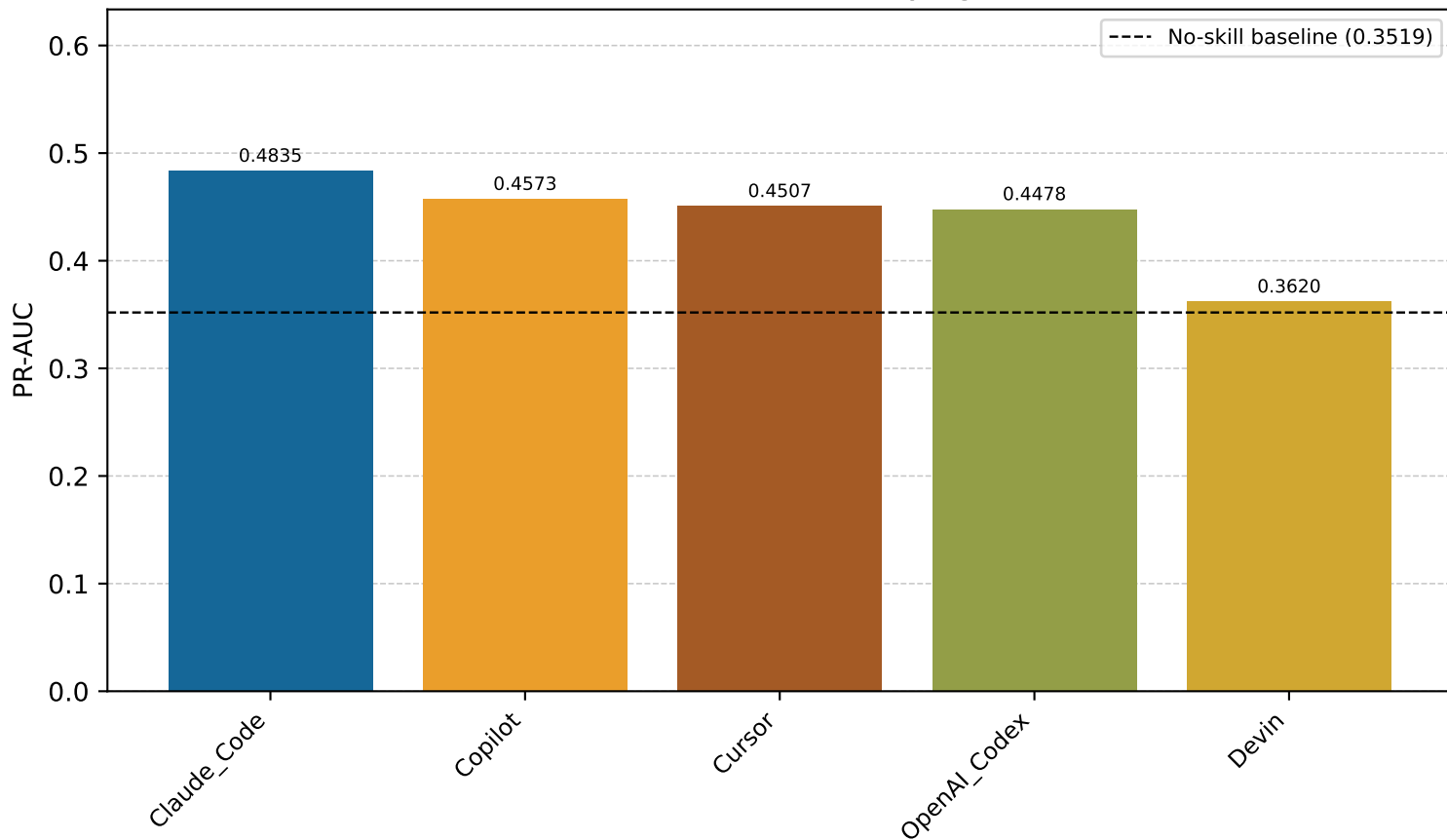
Qwen3 Standard LLM PR-AUC by agent — Test
