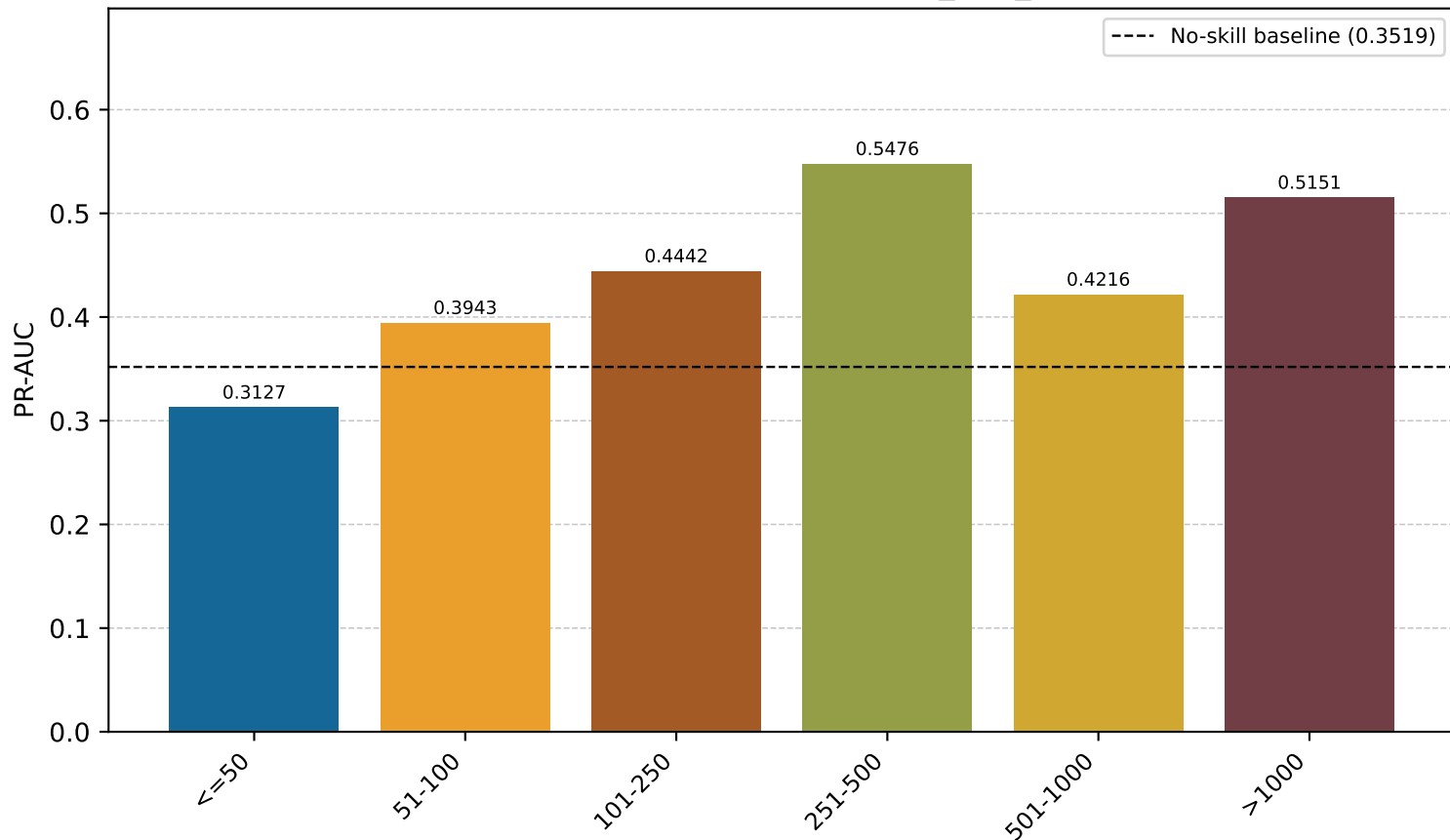
Qwen3 Standard LLM PR-AUC by diff_size_bin — Test
