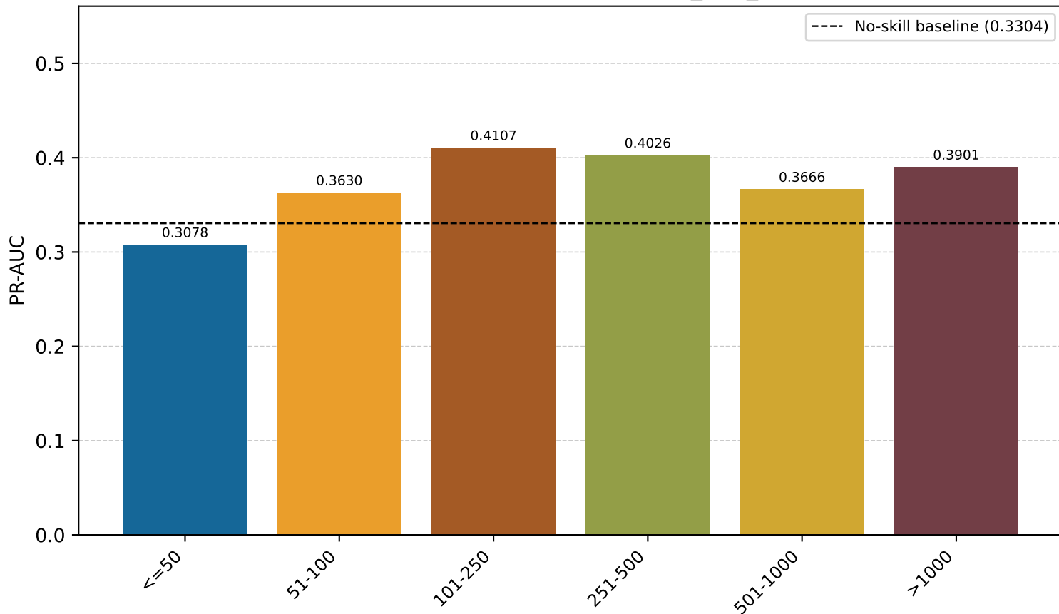
Qwen3 Standard LLM PR-AUC by diff_size_bin — Val
