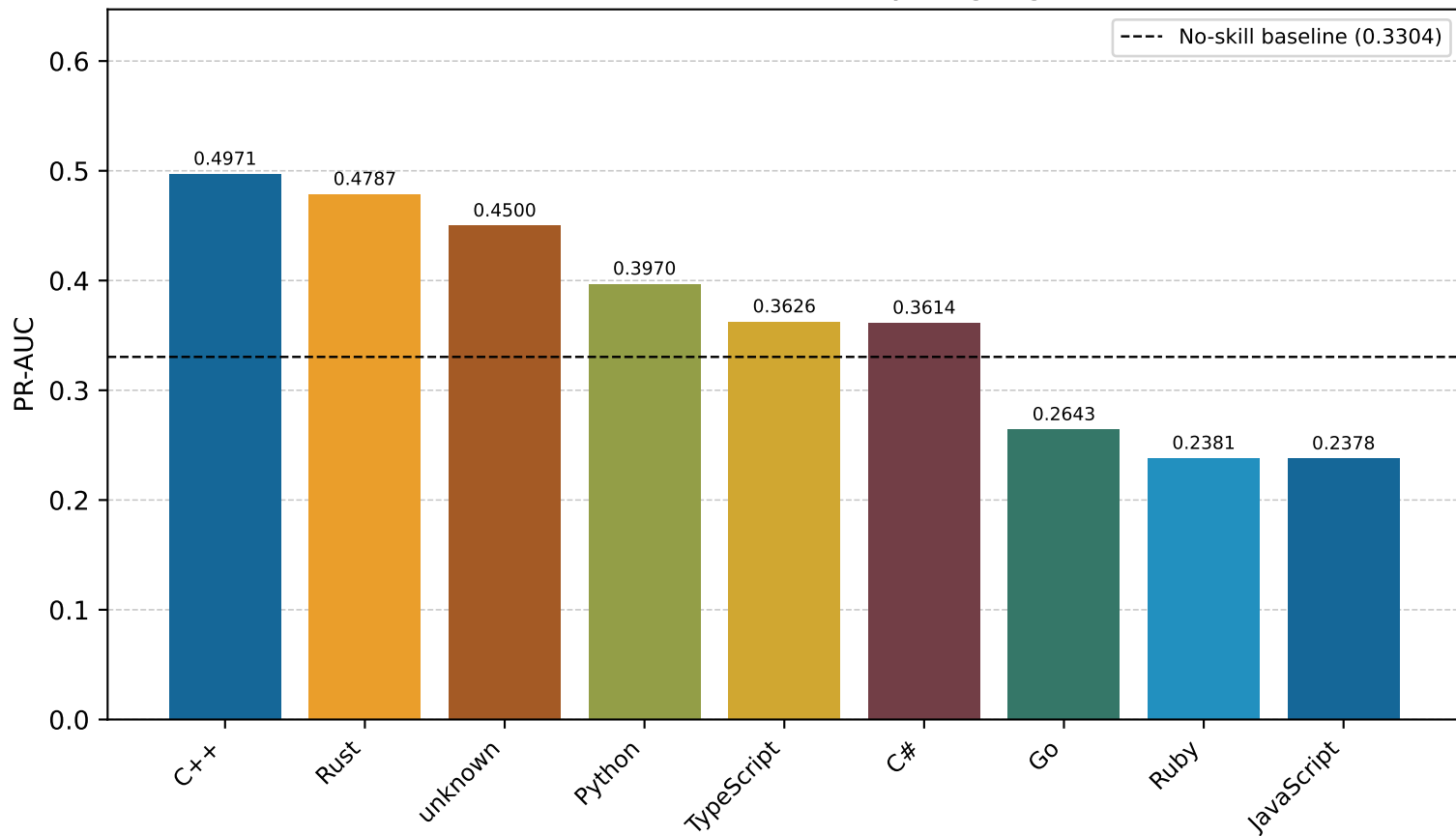
Qwen3 Standard LLM PR-AUC by language — Val
