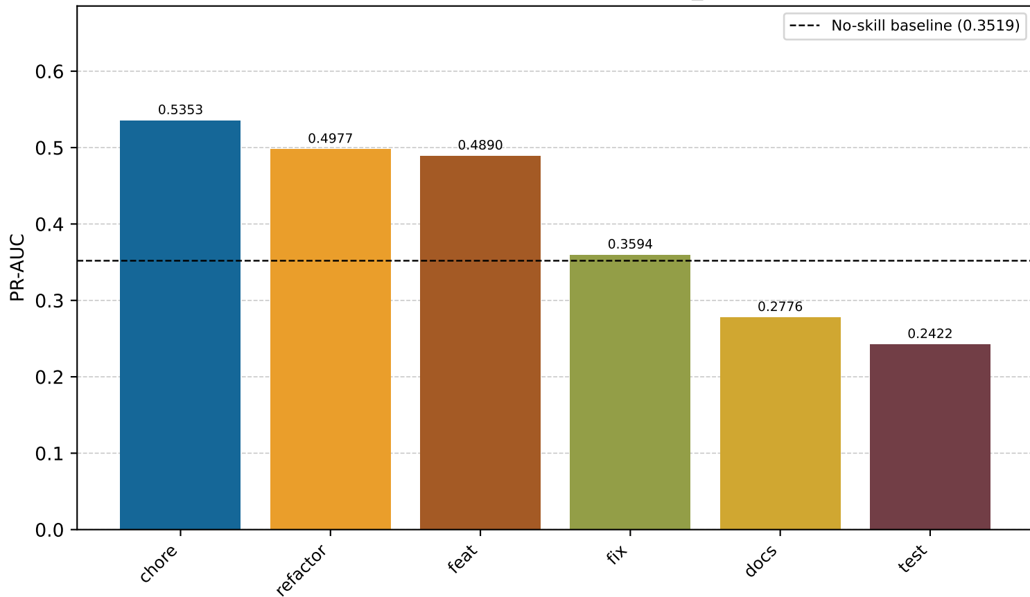
Qwen3 Standard LLM PR-AUC by task_type — Test
